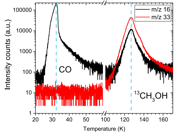
Fig. 2. Desorption profile of the 1:24 13 CH 3 OH:CO mixture, heated at 1 K min -1 . CO is traced by m/z 16 (black) and desorbs just above 30 K, while 13 C-methanol is traced by m/z 33 (red) and desorbs around 130 K. The presence of m/z 16 at the methanol desorption peak is due to the 13 CH 3 (= 16 amu) fragment.
