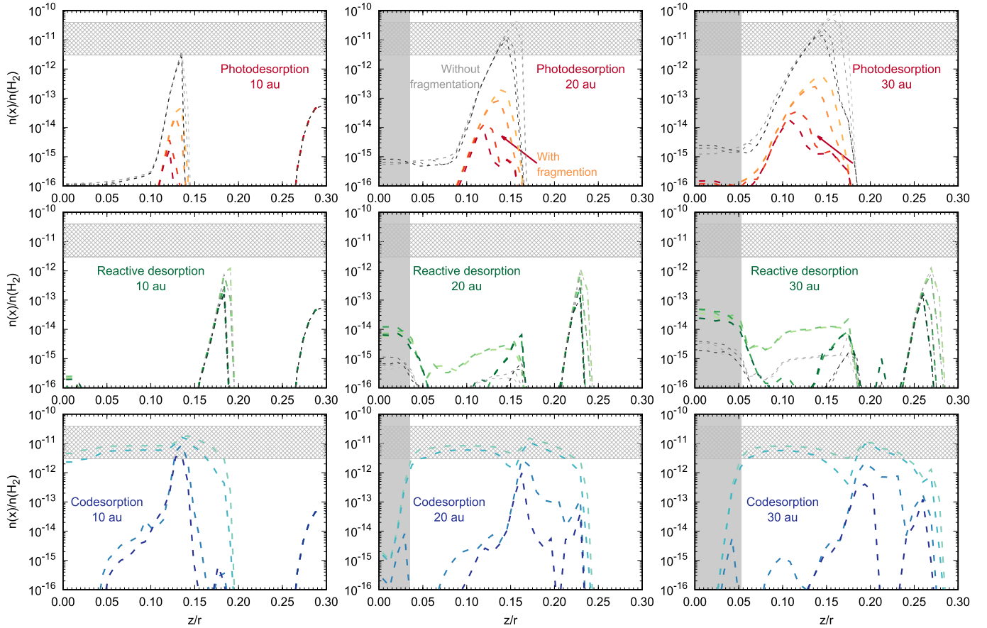
Fig. 6. Fractional abundance of methanol gas as a function of z/r for radii of 10 (left), 20 (middle), and 30 (right) au. Results are shown for three different non-thermal desorption mechanisms: photodesorption only (top), reactive desorption only (middle), and codesorption with CO only (bottom). The colour gradient from light to dark represents four different time steps: 0.5, 1.0, 5.0, and 10 Myr. The grey lines in the top and middle plots represent the “fiducial” model as described in the text (i.e. photodesorption of intact methanol with a yield of \sim 10^{-3} and a reactive desorption probability of 1%). The vertical grey lines in the plots at 20 and 30 au mark the CO snow surface (see Fig. 8). The horizontal bar indicates the methanol abundance as observed towards TW Hya by Walsh et al. (2016).
