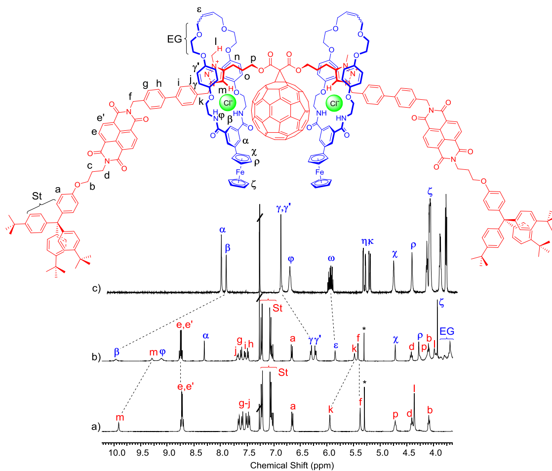
Figure 2. Comparison of ^1\text{H} NMR spectra of a) axle component \mathbf{1}(\text{Cl})_2 , b) [\mathbf{3}]\text{rotaxane } \mathbf{3}(\text{Cl})_2 and c) ferrocenyl-isophthalamide macrocycle precursor \mathbf{2} provides evidence for the dominant co-conformation of [\mathbf{3}]\text{rotaxane } \mathbf{3}(\text{Cl})_2 as depicted above ( \text{CDCl}_3 , 298 K, 400 MHz). Additional proton signals: St = axle stopper, EG = macrocycle ethylene glycol and * = trace residual solvent.
