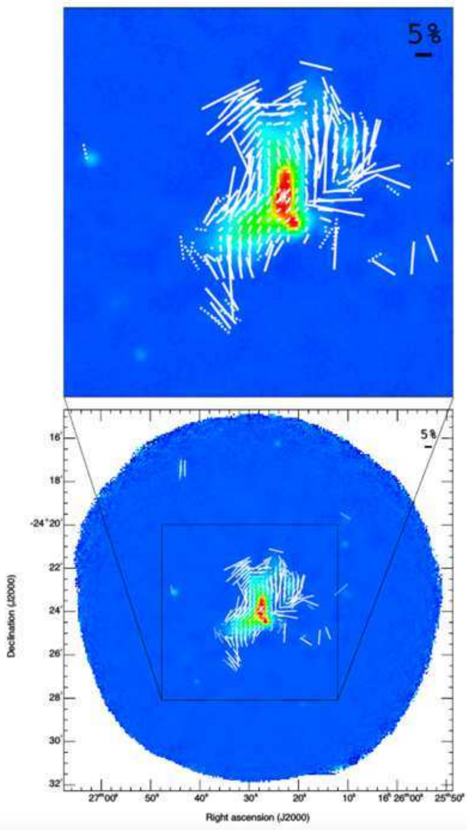
Figure 3. The 850\ \mu\text{m} polarization vector maps. The vectors are sampled on a 12'' grid ( 3 \times 3 pixel smoothing) and plotted where I > 0 , P/\delta P > 2 , and \delta P < 4\% (dotted vectors) and I > 0 , P/\delta P > 3 , and \delta P < 4\% (solid vectors), respectively.
