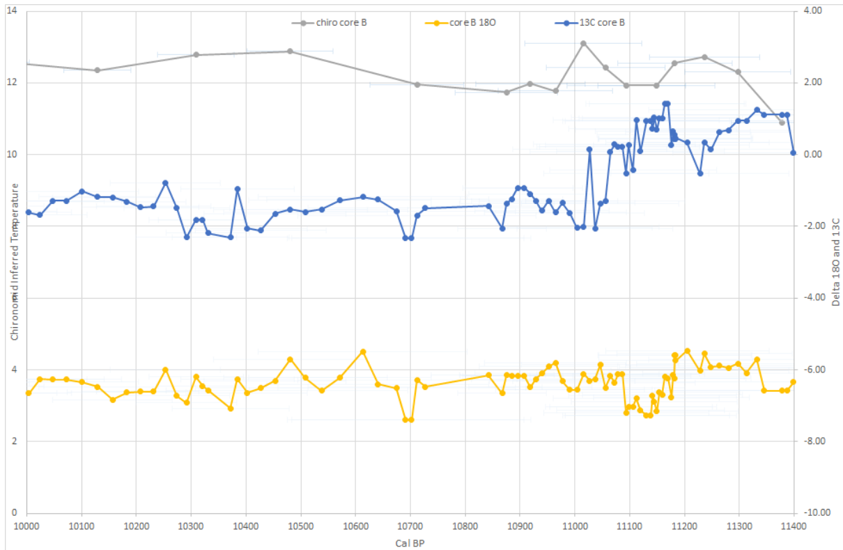
Supplementary Figure 11 CI-T and \delta^{18}\text{O} and \delta^{13}\text{C} from core B against depth in core for the Early Holocene covering ACE 2 and the carbon isotope shift.
