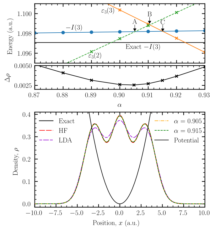
FIG. 1. Upper: The variation in hybrid ionization energy I(3) [ =A(2) ], exact I(3) [ =A(2) ], \epsilon_3(3) , and \epsilon_3(2) with \alpha are illustrated for three electrons in a harmonic oscillator with \omega = 0.25 , an exchange-dominated system. Energies are in Hartree atomic units. There are three "crossing points": (A) A-LUMO, (B) HOMO-LUMO, and (C) I -HOMO. Center: The integrated absolute error in the density \Delta\rho is shown for each value of \alpha . This is defined as \int |\rho^{\text{EXT}}(x) - \rho^{\text{HYB}}(x)| dx , where the \rho^{\text{EXT}} and \rho^{\text{HYB}} correspond to the exact and hybrid densities. Lower: The densities for crossings (A) and (C) are benchmarked against the exact, LDA, and HF cases; the hybrid, HF, and exact curves lie close together.
