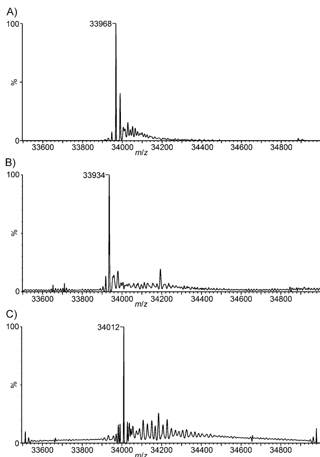
Figure 1. Deconvoluted ESI-mass spectra of A) the K165C variant of S. aureus NAL, B) the K165C variant after 1.5 h treatment with 2,5-dibromo-1,6-hexadiamide, the mass found (33934 \pm 0.63 Da) corresponds exactly with that expected (33934 Da) for the K165Dha enzyme, and C) the K165Dha enzyme after reaction with 2-aminoethanethiol to generate the K165- \gamma -thialysine enzyme. The molecular mass found (34012 \pm 0.16 Da) corresponds exactly with that expected (34012 Da) for the chemically modified enzyme. (See Figure S3 for m/z spectra).
