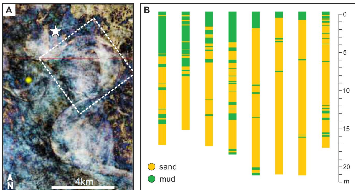
Figure 1: (A) seismic time slice through the meander-belt deposits discussed in the text; the ‘central’ point-bar unit is contained in the hatched frame; the ‘northern’ point-bar unit is located by the star. Location and stratigraphic context undisclosed because of confidentiality. (B) Facies logs from eight of the wells drilled in the northern point-bar body; only the interval interpreted as point-bar deposits is represented.
