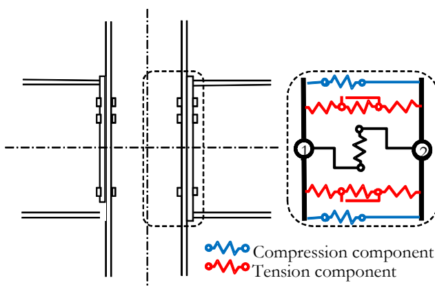
Fig. 1. Component assembly.
