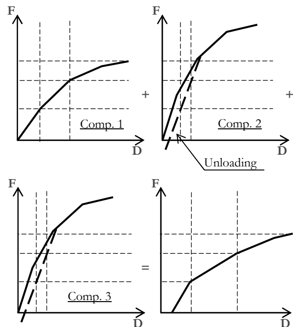
Fig.2. Assembly of the components of a tension bolt row.
