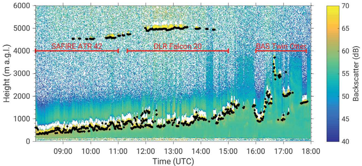
Fig. 7. Time–height evolution of backscatter (color coded) and cloud-base height from ceilometer (black dots) in Savè on 5 Jul 2016. Cloud bases are observed as the thin layer of high backscatter.
