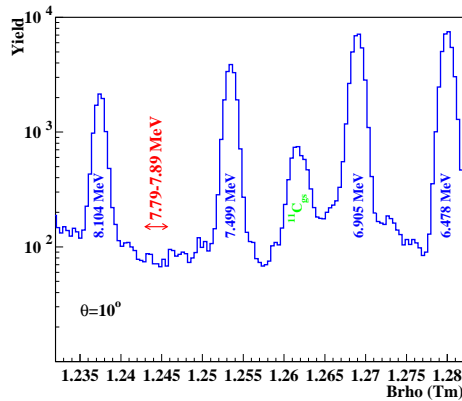
Figure 3. ^{11}\text{C} B\rho position spectrum measured at 10^\circ .
