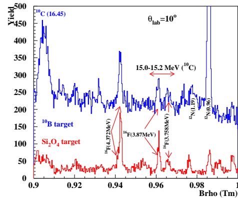
Figure 4. ^{10}\text{C} B\rho position spectrum measured at 10^\circ .
