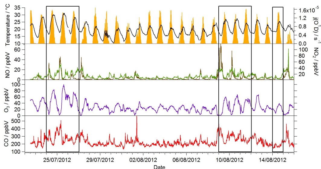
Figure 1. Observed temperature (black line), j(\text{O}^1D) (yellow area), NO (brown line), \text{NO}_2 (green line), \text{O}_3 (purple line) and CO (red line) mixing ratios during the summer ClearLo IOP. Data time resolution is 15 min. Periods of easterly flow are highlighted with the black boxes.
