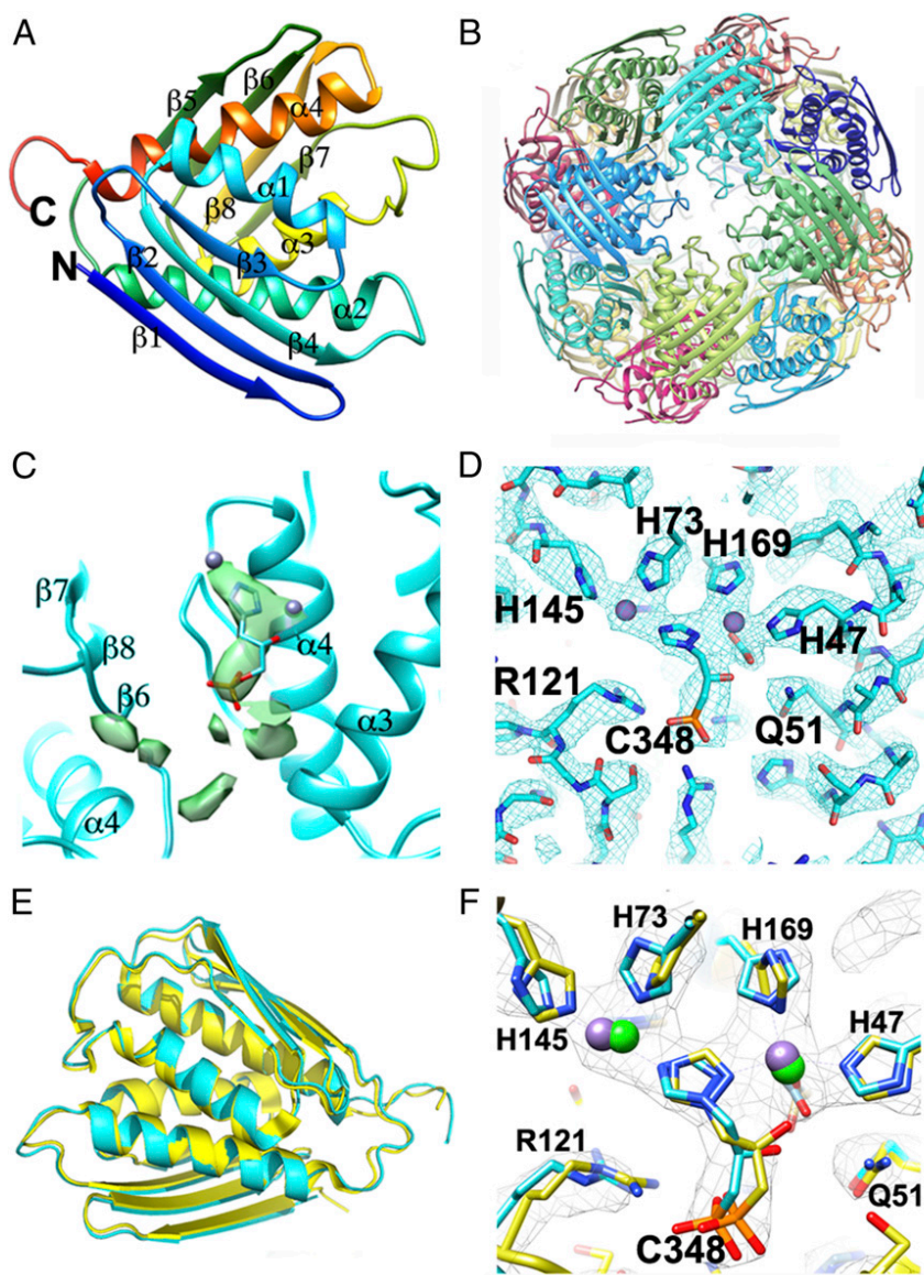
Fig. 2. Analysis of the inhibitor binding pocket and comparison with a representative crystal structure of At_IGPD . (A) Ribbon diagram showing the final model of the At_IGPD monomer colored blue to red from N to C termini, with secondary structure labeled. (B) Ribbon diagram of the full At_IGPD 24-mer, with each subunit colored differently. (C) Positive density within the difference map (green surface) generated by subtracting the map of the de novo built At_IGPD structure from the At_IGPD EM map. This resulted in strong density only within the active site and flanking region, with no other area of significant density not accounted for by the de novo built model. The inhibitor, C348, is shown as sticks, with blue carbon atoms within the difference map. Note that C348 sits within a subunit interface, with the pocket partly formed by \alpha 4 from two different subunits. (D) Fitting of C348 within the active site of IGPD, showing strong density that accommodates both the inhibitor and the two Mn^{2+} ions (purple spheres). (E) A superposition of the At_IGPD structure as derived from EM (blue) and X-ray crystallography [yellow; PDB ID: 5EKW (5)], shown in ribbon format. The conformation of the secondary structure elements within monomer is largely identical, with only minor conformational differences observed within the loop regions. (F) The inhibitor binding pocket of the EM and X-ray crystallography-derived models, colored as in E with key residues and inhibitor shown in stick format. Mn^{2+} ions are shown as purple (EM) or green (X-ray) spheres. In all parts, nitrogen, oxygen, and phosphorous are colored blue, red, and orange, respectively.
