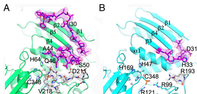
Fig. 4. Insertion loop in Sc _IGPD. ( A ) The 24-residue insertion loop in Sc _IGPD, situated between \beta 2 and \beta 4 colored in purple and the C-terminal inhibitor/substrate binding loop is shown in gray. The insertion (purple) within Sc _IGPD lies next to the C-terminal substrate/inhibitor binding loop (gray), possibly stabilizing the interaction. The 24-residue insert in Sc _IGPD compared with At _IGPD forms an additional \beta -strand ( \beta 3 ) between A44 and Q46, and therefore there is one extra strand within its external \beta -sheet. Residues between K38 and A44 are not well resolved within the EM map, and have not been modeled, and some residues in the loop region have been truncated because of poor side chain density. ( B ) The equivalent view in At _IGPD with a much smaller loop between \beta 2 and \beta 3 , which is well defined in the EM map (shown in purple). The C-terminal loop (gray) is more poorly defined and makes no interactions with the loop region between \beta 2 and \beta 3 .
