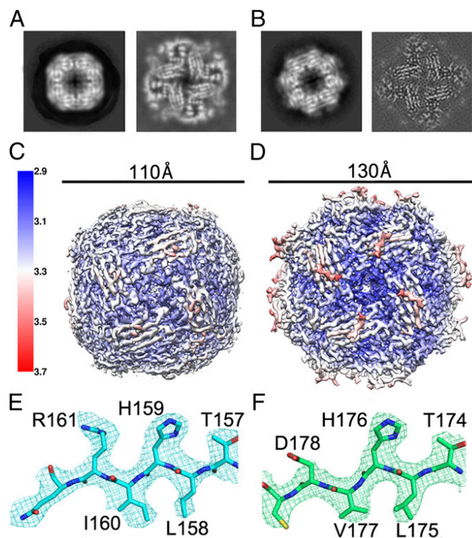
Fig. 1. The cryo-EM structure of both At IGPD and Sc IGPD. Representative 2D class average ( Left ) and a slice through from the final 3D reconstruction showing the internal \beta -strands ( Right ) for At IGPD ( A ) and Sc IGPD ( B ). 3D reconstruction colored by local resolution (determined within RELION) for At IGPD ( C ) and Sc IGPD ( D ) (color key is shown on the right and approximate dimensions above). Example of the density in the EM maps for the equivalent region in At IGPD ( E ; blue carbon atoms) and Sc IGPD ( F ; green carbon atoms); note the different shape of the density for the Ile ( At IGPD) and Val ( Sc IGPD) residue. In E and F , nitrogen, oxygen, and sulfur atoms are colored blue, red, and yellow, respectively.
