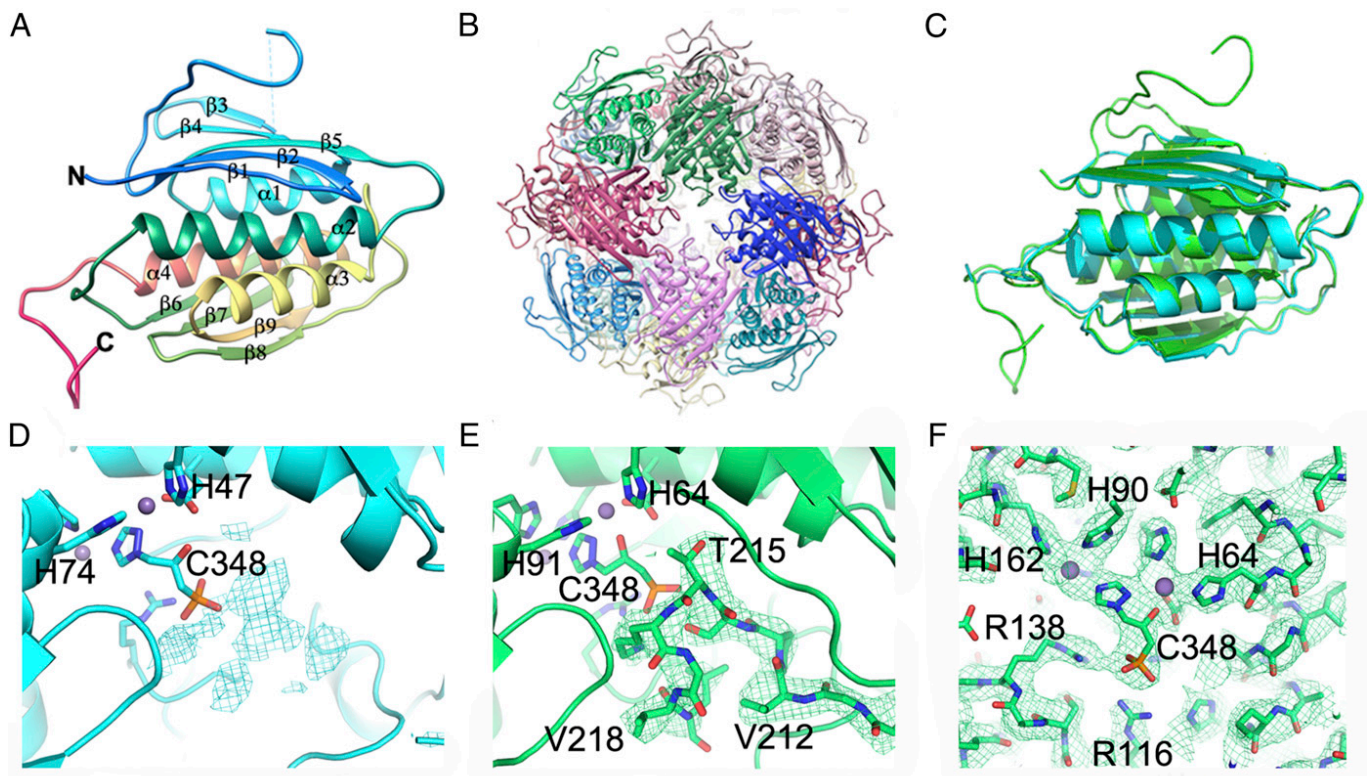
Fig. 3. Analysis of the Sc_IGPD structure and comparisons to At_IGPD . ( A ) A ribbon diagram of the Sc_IGPD monomer colored blue to red from the N to C termini and with secondary structure labeled. ( B ) Ribbon diagram of the full At_IGPD 24-mer, with each subunit colored differently. ( C ) Superposition of the At_IGPD (blue) and Sc_IGPD (green) structures, shown in ribbon format, with the additional 24-residue loop region in the later shown above the N-terminal \beta -sheet. ( D ) Density within the At_IGPD EM map around the C-terminal domain showing weak density for this region. ( E ) The C-terminal loop region of Sc_IGPD , which can be unambiguously assigned within the EM map. Both D and E are shown in an equivalent view with the same map contouring level. ( F ) Fitting of C348 within the active site of IGPD, showing strong density that accommodates the inhibitor, surrounding residues, and the two Mn^{2+} ions (purple spheres).
