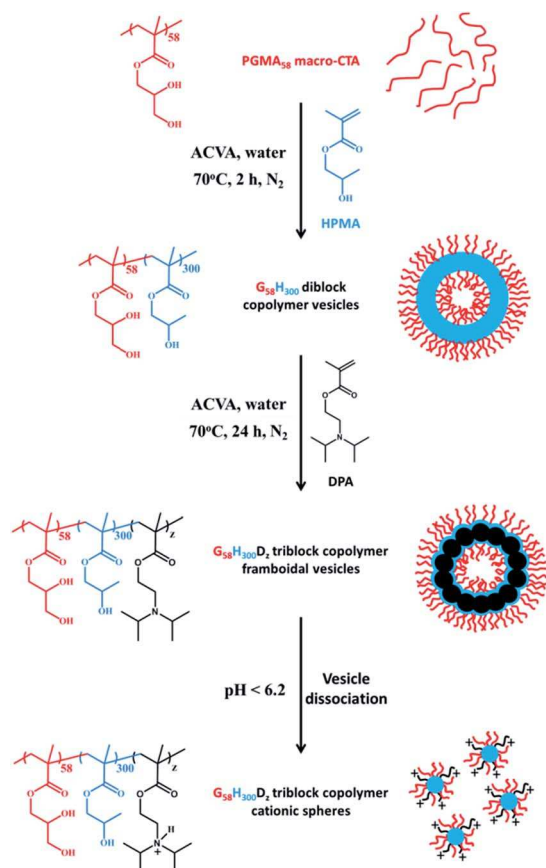
Fig. 1 Synthetic route to PGMA_{58} - PPHMA_{300} - PDPA_z ( G_{58}H_{300}D_z ) framboidal triblock copolymer vesicles via polymerisation-induced self-assembly (PISA) in aqueous solution at pH 7–8. Addition of acid causes protonation of the tertiary amine residues, which renders the PDPA block hydrophilic and induces vesicle dissociation. Inset: schematic cartoon of precursor vesicles, framboidal vesicles and cationic spheres.
