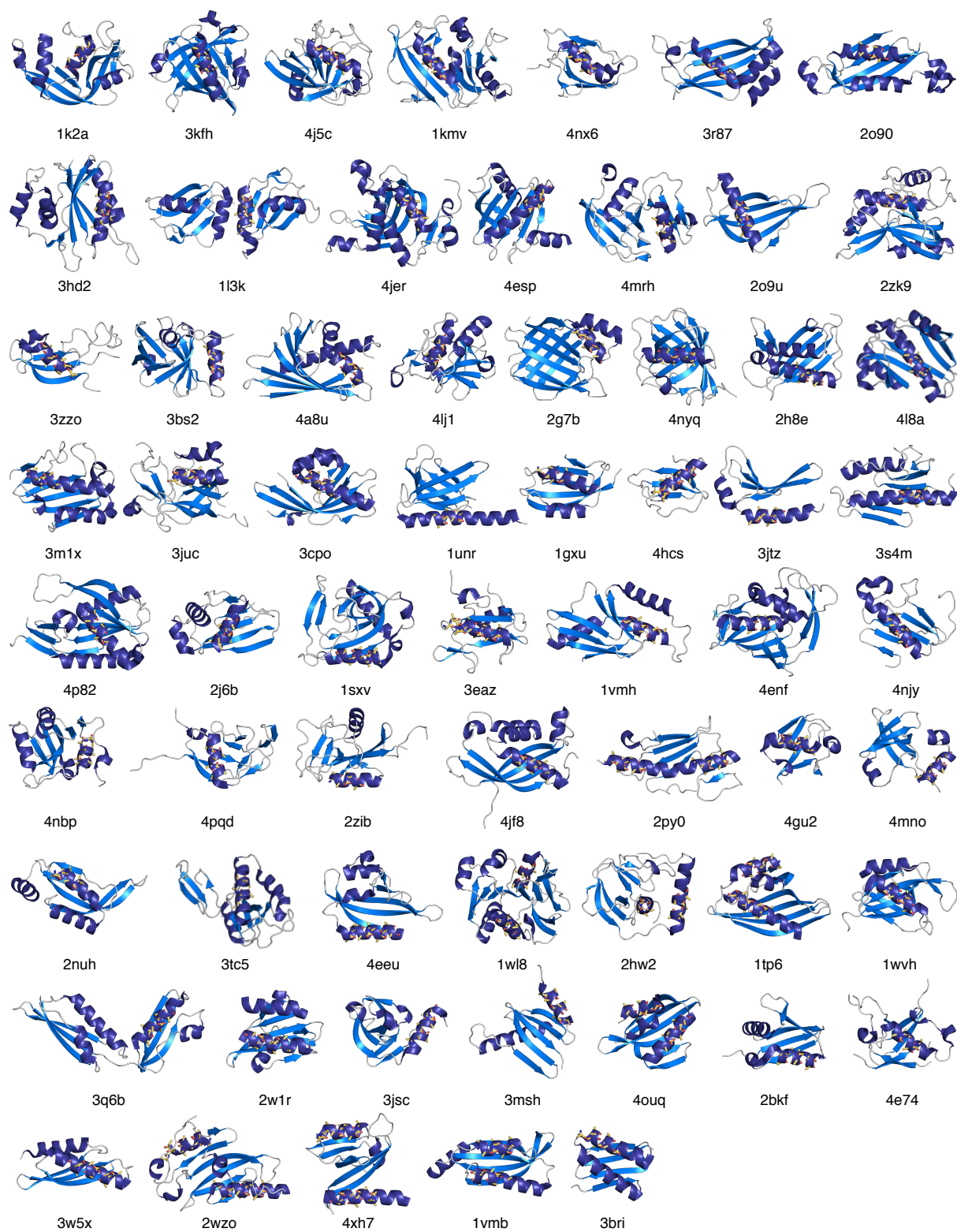
Figure 1 Test cases in the mixed \alpha/\beta test set solved by Fragon . The fragment placed by Phaser is shown as yellow sticks.
