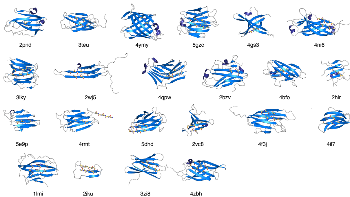
Figure 2 Test cases in the all- \beta test set solved by Fragon . The fragment placed by Phaser is shown as yellow sticks.
