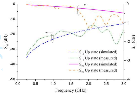
Fig. 6. MEMS Aluminum varactor return and transmission loss UP state response.
