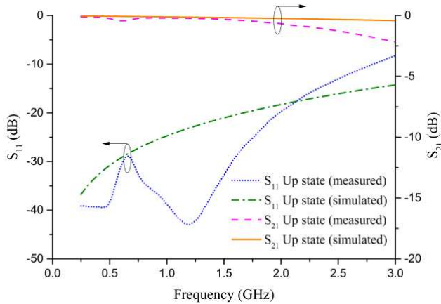
Fig. 4. MEMS Aluminum switch return and transmission loss UP state response.
