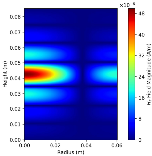
Fig. 7. Plot of the magnitude of the H_z -field inside the aperiodic Bragg resonator at 10.02 GHz.
