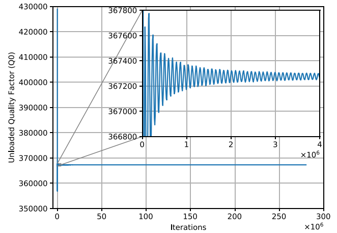
Fig. 4. Simulated quality factor of the aperiodic Bragg resonator. The Q-factor was calculated using the perturbation method after every 10000 time steps of the FDTD-BOR solver.
