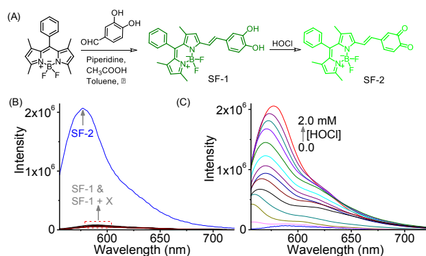
Figure 1. (A) Methodologies adopted for synthesis of SF-1 ; (B) change in emission spectra of SF-1 in the absence and presence of different ROS/NOS species (HOCl, X: \text{H}_2\text{O}_2 , \cdot\text{OH} , \text{Na}_2\text{S}_2 , \text{HNO} , Tyrosinase, Cysteine, \text{NO}_3^- , \text{NO}_2^- , \text{Fe}^{2+} , \text{Fe}^{3+} , \text{Cu}^{2+} , \text{Cr}^{3+} , \text{Hg}^{2+} , \text{Zn}^{2+} and \text{K}^+ ); (C) emission titration profile for SF-1 in the presence of varying concentration of HOCl; All emission spectra were recorded using \lambda_{\text{ex}} = 550 \text{ nm} in aq. PBS buffer-acetonitrile (9:1, v/v) solution.
