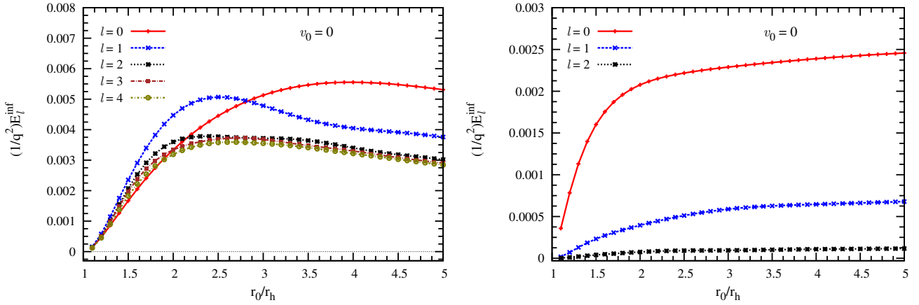
Fig. 6 Numerical estimates of the emitted energy radiated to infinity, E_l^{\text{inf}} , as a function of r_0 , obtained using Eq. (28), considering Eq. (34) (plots on the left) and Eq. (35) with B = 0 (plots on the right), for selected choices of multipole numbers obtained from Eq. (28).
