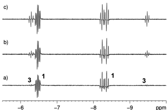
Figure 3. Hydride region of a series of \{^1\text{H}\} NMR spectra of a solution of 1 in \text{C}_6\text{D}_6 in the presence of a 10-fold excess of \text{AsPh}_3 under p\text{-H}_2 at room temperature showing hyperpolarized signals for 1 and 3 after (a) 1 laser shot, (b) 2 laser shots, and (c) 4 laser shots.
