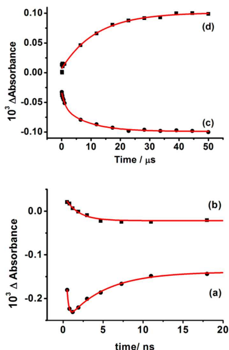
Figure 12. Kinetic plots observed after photolysis of 1 under Ar (plots (a) and (b) on a nanosecond time scale and plots (c) and (d) on a microsecond time scale): (a) 1939\text{ cm}^{-1} assigned to 1 which shows a rapid increase, followed by a bleach recovery, \tau = 4.8 \pm 0.4\text{ ns} ; (b) 1951\text{ cm}^{-1} , \tau = 1.7 \pm 0.4\text{ ns} ; (c) 1938\text{ cm}^{-1} assigned to 1 , \tau_1 = 1.1 \pm 0.4\text{ }\mu\text{s} , \tau_2 = 9 \pm 2\text{ }\mu\text{s} ; (d) 1970\text{ cm}^{-1} assigned to the dimeric species, \tau = 12 \pm 2\text{ }\mu\text{s} . \Delta\text{Absorbance} values have been normalized.
