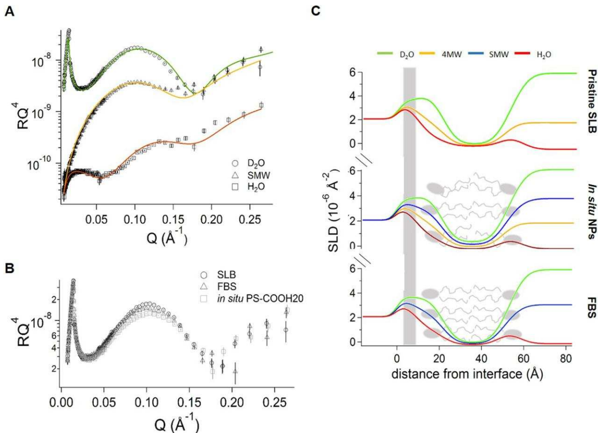
Figure 5. The structural effects on the SLB after exposure to in situ PS-COOH 20 NPs and 55% FBS solutions observed by NR experiments. A) NR data (symbols) of the pristine SLB and fitting curves (lines) obtained by simultaneous co-refinement of the NR curves at three contrasts ( D_2O , SMW, H_2O ) to the 5-slab model described in the text. B) NR data (symbols) of the pristine SLB, after treatment with a solution of 55% FBS and after treatment with in situ NPs (see legend). C) SLD profile of the pristine SLB (top), of the SLB treated with in situ NP (middle) and of the SLB treated with 55% FBS (bottom).
