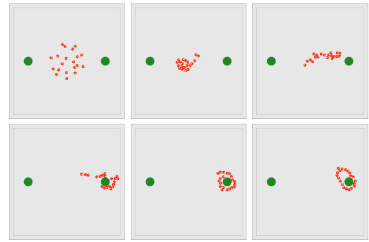
Fig. 3. Sequence of snapshots showing a swarm of 20 simulated robots choosing option B . They were taken (from the top left to the bottom right) once 0, 10, 20, 30, 40, and 300 s had elapsed. Initially the swarm aggregates around the center of the arena. The motion of the robots causes symmetry-breaking and as a result the swarm collectively approaches the option on the right. When t = 40 s the robots orbit around option B and remain committed to their choice.
