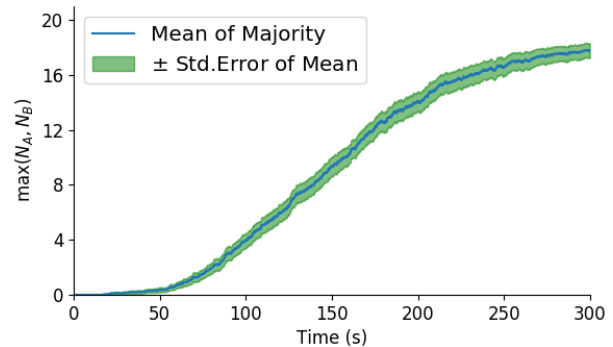
Fig. 11. Dynamics of \max(N_A, N_B) , averaged over the 50 experimental trials with 20 physical robots.
