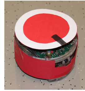
Fig. 8. Close view of the robotic platform used in the experiments. The e-puck is coated in red to be identifiable by other e-pucks. The marker on its top is used by the tracking system for the post-analysis.
