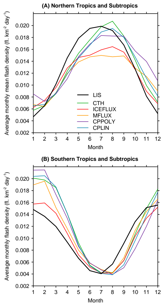
Figure 8. Five-year climatological annual cycle of flash density for 2007–2011 for (a) the northern region ( 0^\circ\text{--}38^\circ N) and (b) the southern region ( 38^\circ S– 0^\circ ). Results are shown for the LIS measurements and the five parametrisations.
