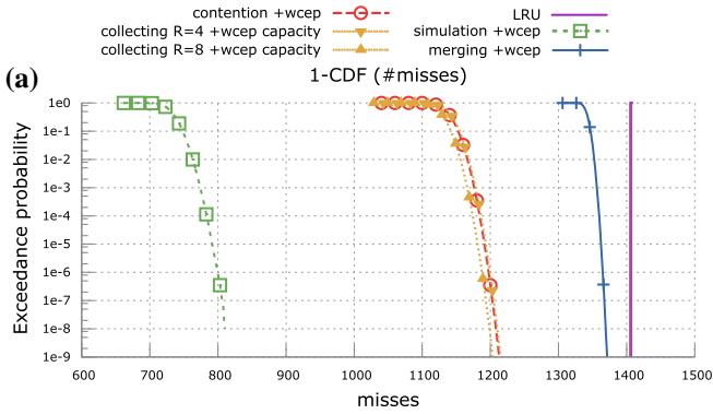
Estimated miss distribution for quart, 77 distinct memory blocks, 1526 accesses on the longest path
