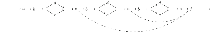
Fig. 5 Simple do-while loop structure (Fig. 4) unrolled assuming \max\text{-iter}(l) = 3 . The unrolled (dashed) back-edges are only kept when a generic loop unrolling algorithm is used. They are removed when \max\text{-iter}(l) iterations are enforced
