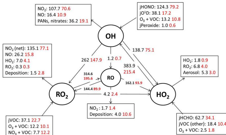
Figure 5. Mean daytime (11:00–15:00 black number and 06:00–21:00, red number) rates of reaction for formation, propagation and termination of radicals in units of 10^5 \text{ molecule cm}^{-3} \text{ s}^{-1} for the whole campaign period.
