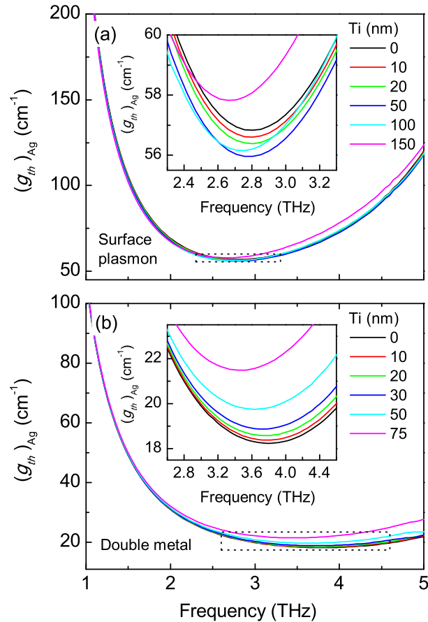
Fig. 4. The room temperature threshold gain as a function of frequency for the Ag-based surface-plasmon waveguide (a) and double metal waveguide (b) with different thickness of Ti adhesion layer. The insets show enlarged figures in the dotted squares.
