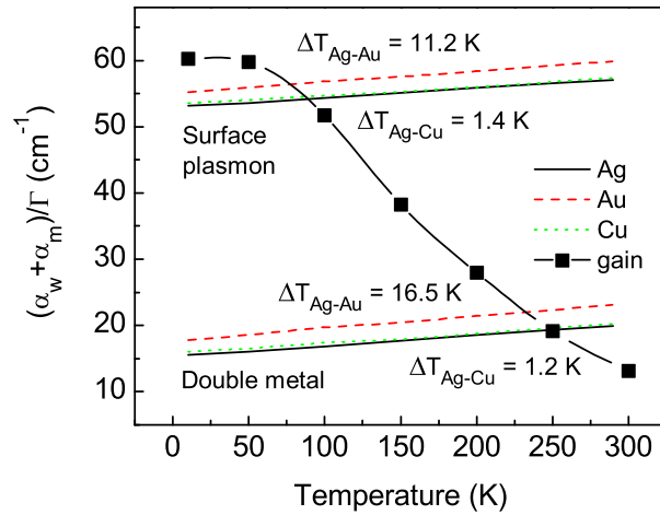
Fig. 2. Temperature evolution of the calculated peak gain (black squares), and the threshold gain for devices with Ag (black solid lines), Au (red dashed lines) and Cu-based (green dots) surface-plasmon waveguides and double metal waveguides. The peak gain is from a 3.1-THz QCL based on a three-well resonant phonon design [14].
