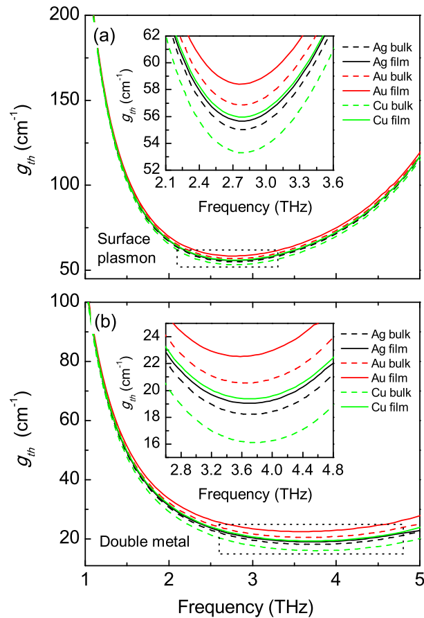
Fig. 6. The room temperature threshold gain as a function of frequency for the Ag, Au and Cu-based surface-plasmon waveguide (a) and double metal waveguide (b). The threshold gains are calculated using the dielectric constants from the metal films and bulk metals, respectively. The insets show enlarged figures in the dotted squares.
