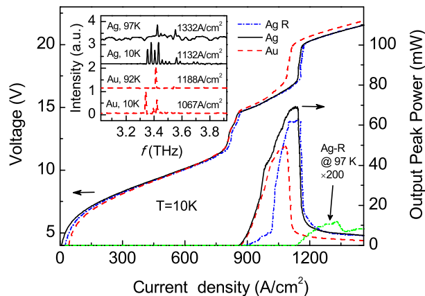
Fig. 8. LIV curves of QCLs (pair A2) with Ag and Au waveguide layers measured at 10 K. The inset shows the emission spectra measured at 10 K and at the maximum operating temperatures. The devices were driven by 2 \mu s-wide current pulses with a duty cycle of 2%. Ag-R indicates the re-characterised LIV curves of the Ag-based device after it had been placed in air for more than two years.
