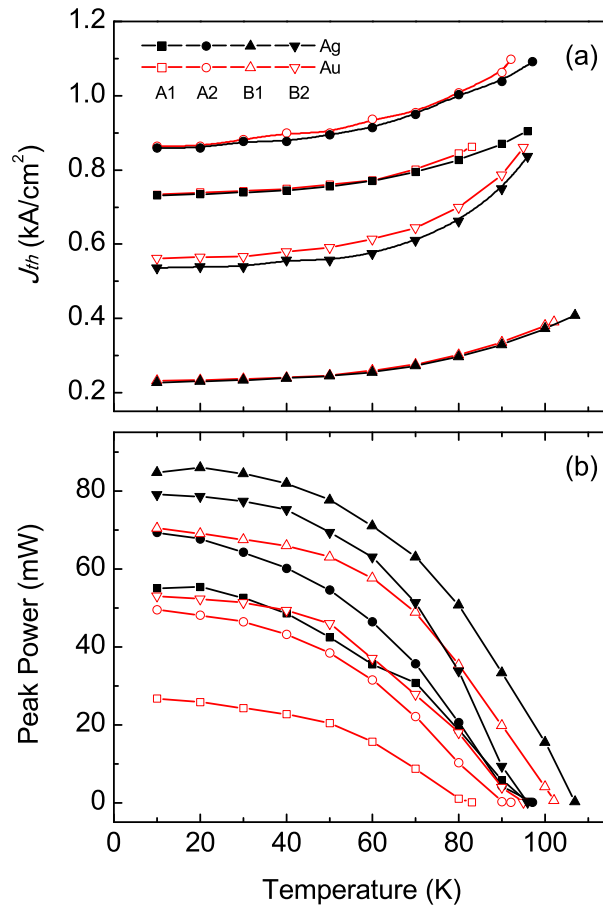
Fig. 7. The threshold current density (a) and peak output power (b) measured from four pairs of QCLs (A1, A2, B1 and B2) as a function of heat-sink temperature. For each pair of devices, the only difference is the waveguide metal layer.
