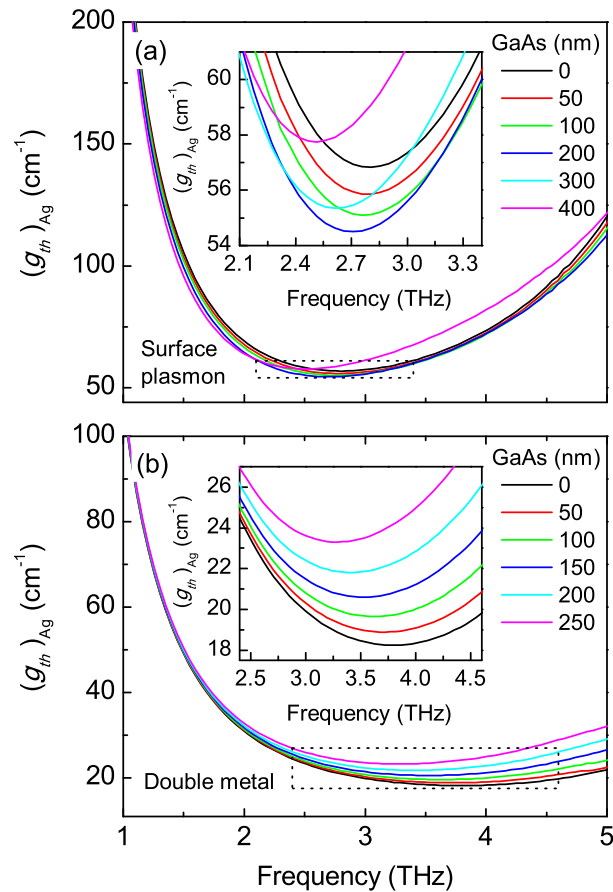
Fig. 5. The room temperature threshold gain plotted as a function of frequency for the Ag-based surface-plasmon waveguide (a) and double metal waveguide (b) with different thickness of GaAs top contact layer. The insets show enlarged figures in the dotted squares.
