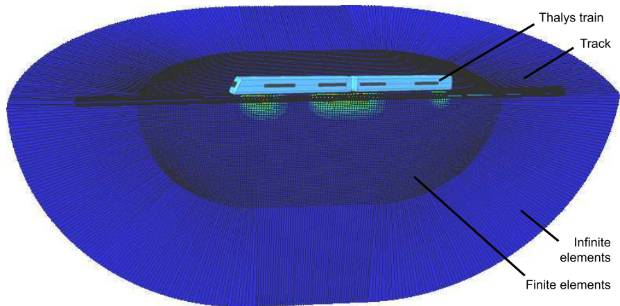
Figure 3. Symmetrical soil finite/infinite element solution
