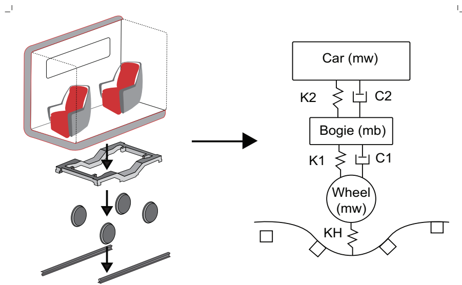
Figure 4. Vehicle modelling - Typical 1/2 Thalys car (left), simplified Thalys model (right)
