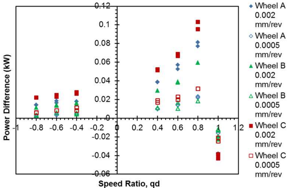
Figure 6 – The average power consumption difference between before and during dressing.
