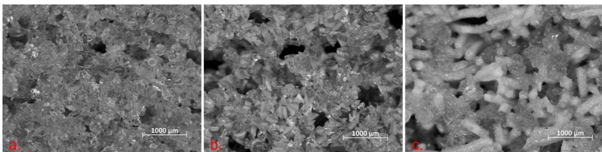
Figure 1 – Micrographs of the three different wheels tested with varying morphology (a) wheel A with conventional grits (b) wheel B containing triangular grits and (c) wheel C containing elongated grits.
