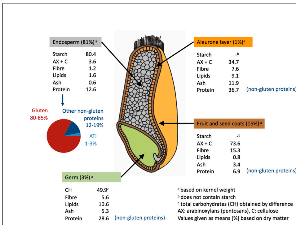
Figure 2. Wheat components.
