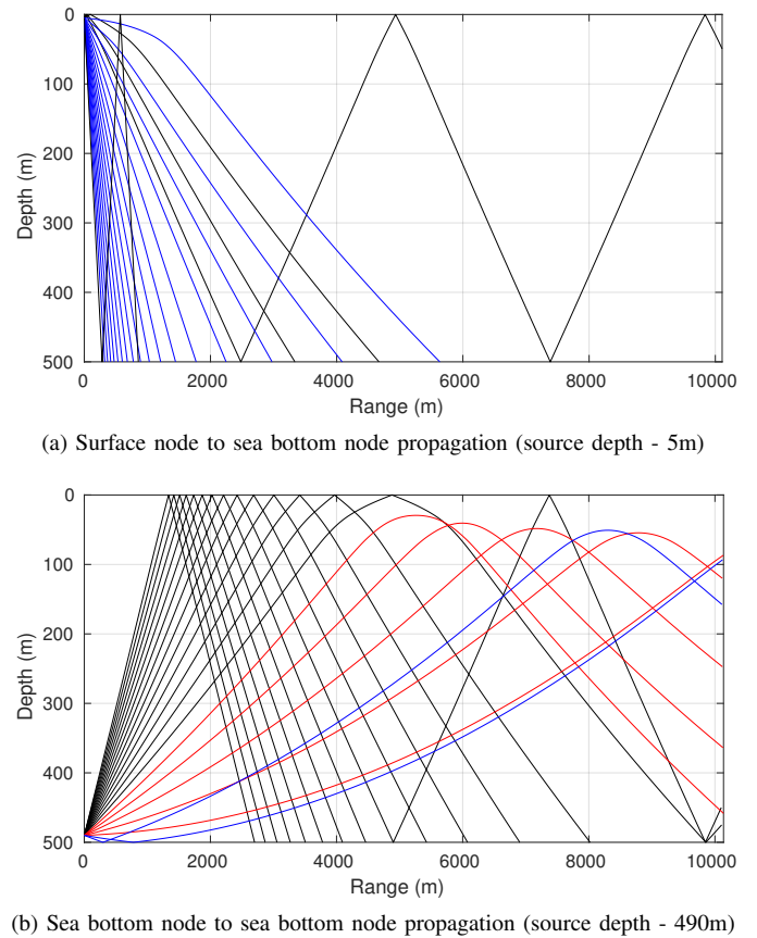
Fig. 3. Acoustic ray trajectories obtained using the BELLHOP simulator
