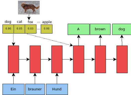
Figure 1: An illustration of our Multimodal NMT system. Departing from usual methods, we replace the lower-level CNN image representation with a vector representing the output of a 1,000-way visual classifier, where each element in the vector represents the estimated posterior probability of an object category occurring in the image. We experiment with conditioning the image representation on either the encoder or the decoder (dashed lines), and also at each source word (not shown in the Figure).
