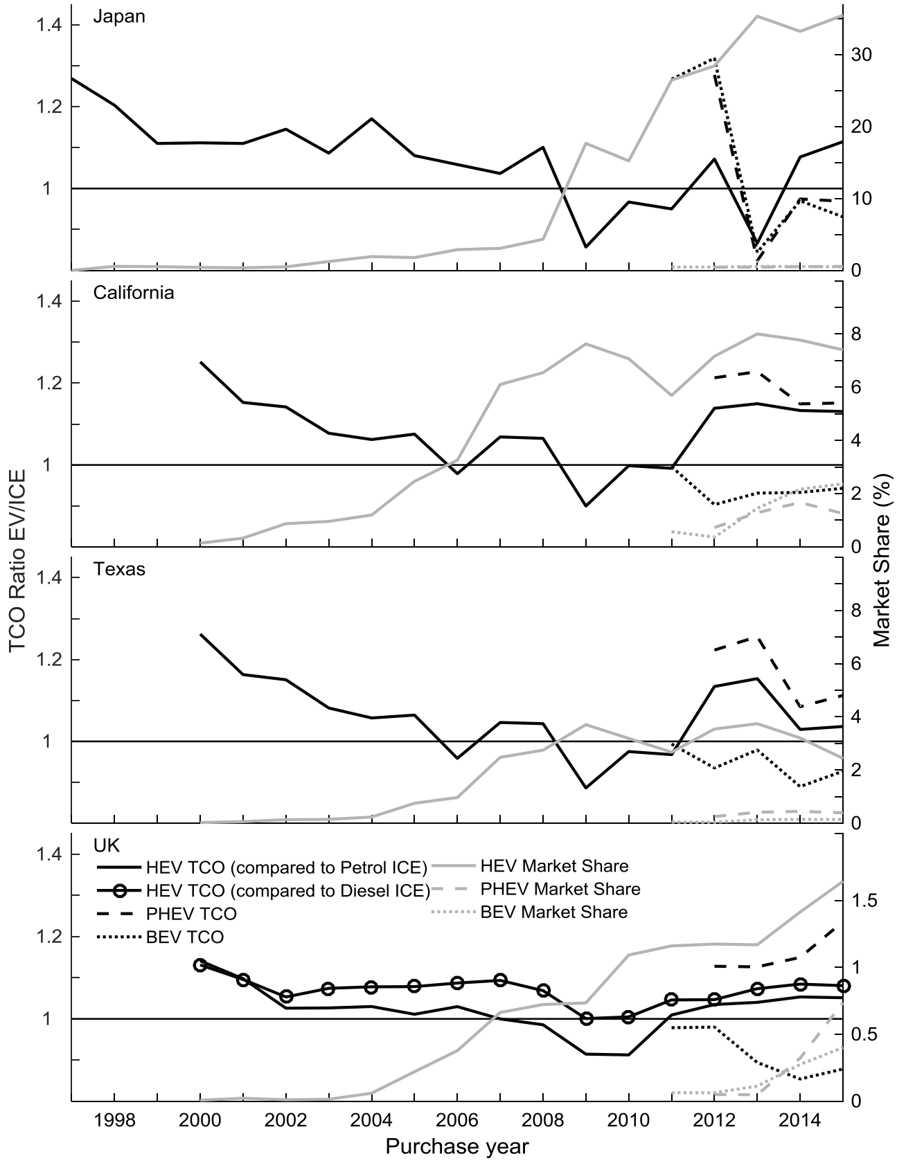
FIGURE 3: TCO ratio and market share for the UK, California, Texas and Japan 1997-2015. [2 column figure]
