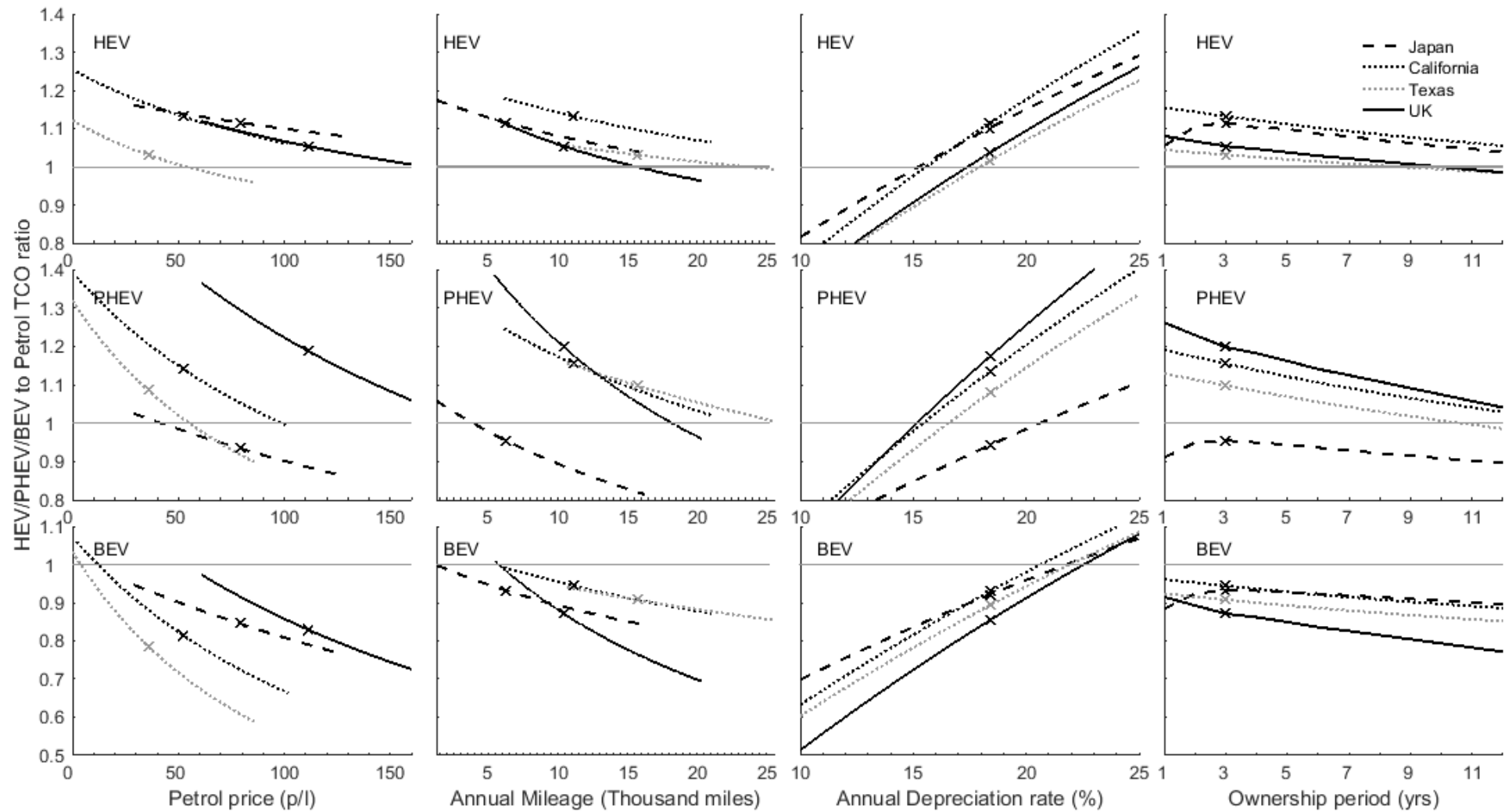
FIGURE 4: TCO Sensitivity Analysis for base year 2015, cross (X) indicates baseline value. [whole page figure]
