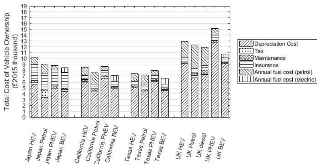
FIGURE 2: TCO component breakdown for 2015 across all regions [single column figure]
