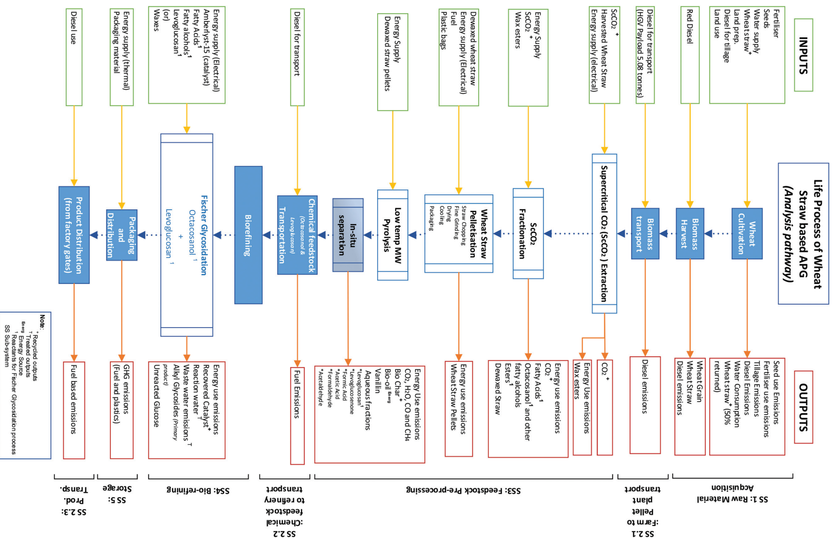
Fig. 1 Cradle-to-gate life cycle stages for WS-APG production.
