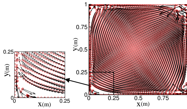
(a) ISPH (diverged at t = 0.53 s)
