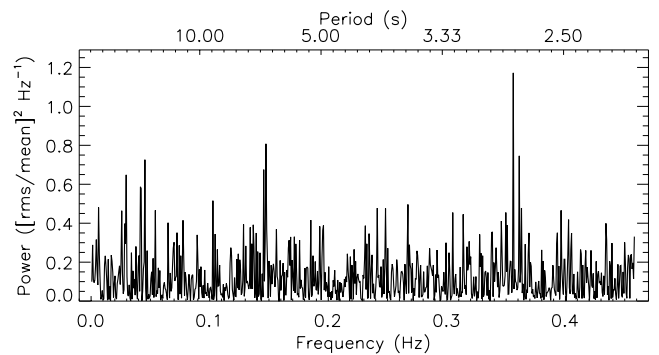
Figure 3. The power spectrum of the ULTRASPEC light curve in fractional \text{rms}^2 units, after correcting for the decay. The minimum period detectable, given the time resolution, is 2.18 s, while the longest time-scale monitored is 1587 s. The peaks in the power spectrum are generated by random noise, see Section 3.1 for more details. The lack of a preferred frequency confirms the smoothness of the light curve.
