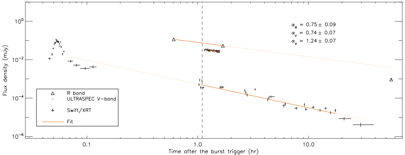
Figure 7. The optical and X-ray afterglow light curves of GRB 080210. The Swift /XRT X-ray light curve (at 1.73 keV) is plotted beneath the optical data. The ULTRASPEC V -band light curve is here plotted with a bin factor of 10. The R -band decay is derived from the VLT/FORS2 data. Late time points were excluded to avoid a possible break. The solid lines show the fit to the data, while the dotted lines extrapolate the fit to the complete data sets. The vertical line shows the SED time. The errors are 1\sigma .
