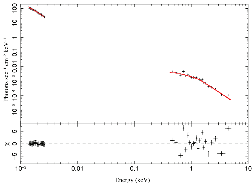
Figure 6. The SED of the optical 300V spectrum (×) and the X-ray spectrum (+), at 66 min after the burst. The solid line shows the best-fitting model, a broken power law with spectral slopes \beta_X = 1.59 \pm 0.11 and \beta_{\text{opt}} = 0.71 \pm 0.02 , for an SMC-type dust extinction, see Table 4. The residuals are displayed in the bottom panel.
