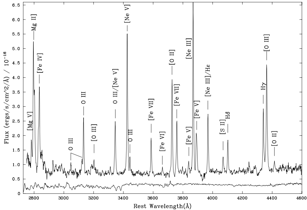
Figure 2. WHT nuclear spectrum of Q1131+16 taken on the ISIS blue arm. Unresolved blends are indicated by an ‘/’, while resolved blends are indicated by an ‘&’. The flux scale is measured in units of 10^{-16} \text{ erg s}^{-1} \text{ \AA}^{-1} \text{ cm}^{-2} . Note the strength of high-ionization lines such as [Ne v] and [Fe vii] relative to [O ii], and of [O iii] \lambda 4363 relative to H \delta . For reference, we also show a scaled version of the night sky spectrum extracted from the 2D frames at the bottom of the plot.
