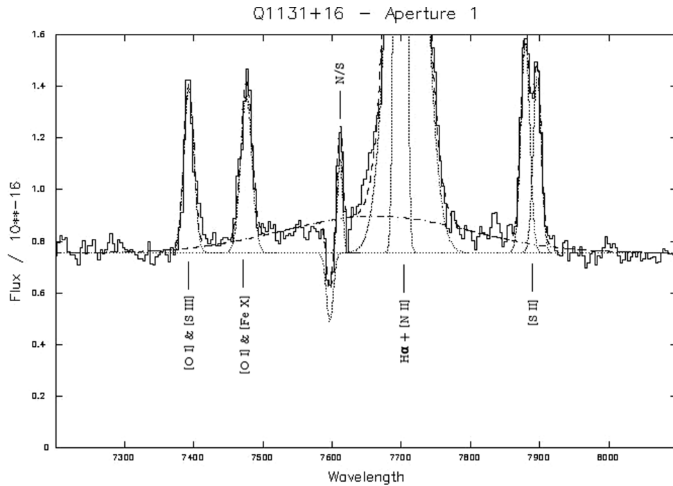
Figure 6. The broad component centred on the H\alpha + [N\text{II}] emission blend. The telluric feature is fitted as well as the various emission components from Q1131+16.
