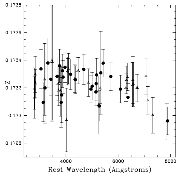
Figure 10. Individual redshifts of the emission lines of Q1131+16 as measured for the WHT data. The triangles indicate the low-ionization emission lines and neutral species emission and the black circles indicate the FHILs. All points lie within 1.5\sigma of the mean redshift; however, the longer wavelength emission lines ([O II] \lambda\lambda 7320, 7330 , [Ar IV] \lambda 7868 and [Fe XI] \lambda 7892 ) do not. This is likely due to larger wavelength calibration errors at the long-wavelength end of the spectrum.
