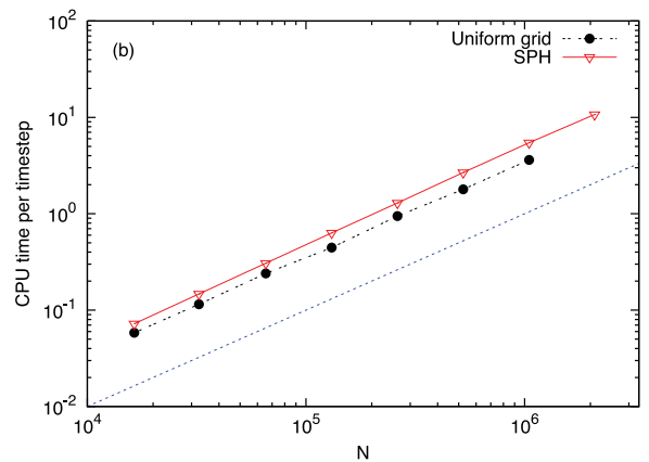
Figure 9. (a) The CPU time per cell–cell, or particle–particle, interaction in the finite volume and SPH codes. (b) The total CPU time of all cells or particles per time-step for the finite volume and SPH codes. The trend expected for constant no. of operations per cell/particle ( t_{\text{CPU}} \propto N ) is shown for reference.
