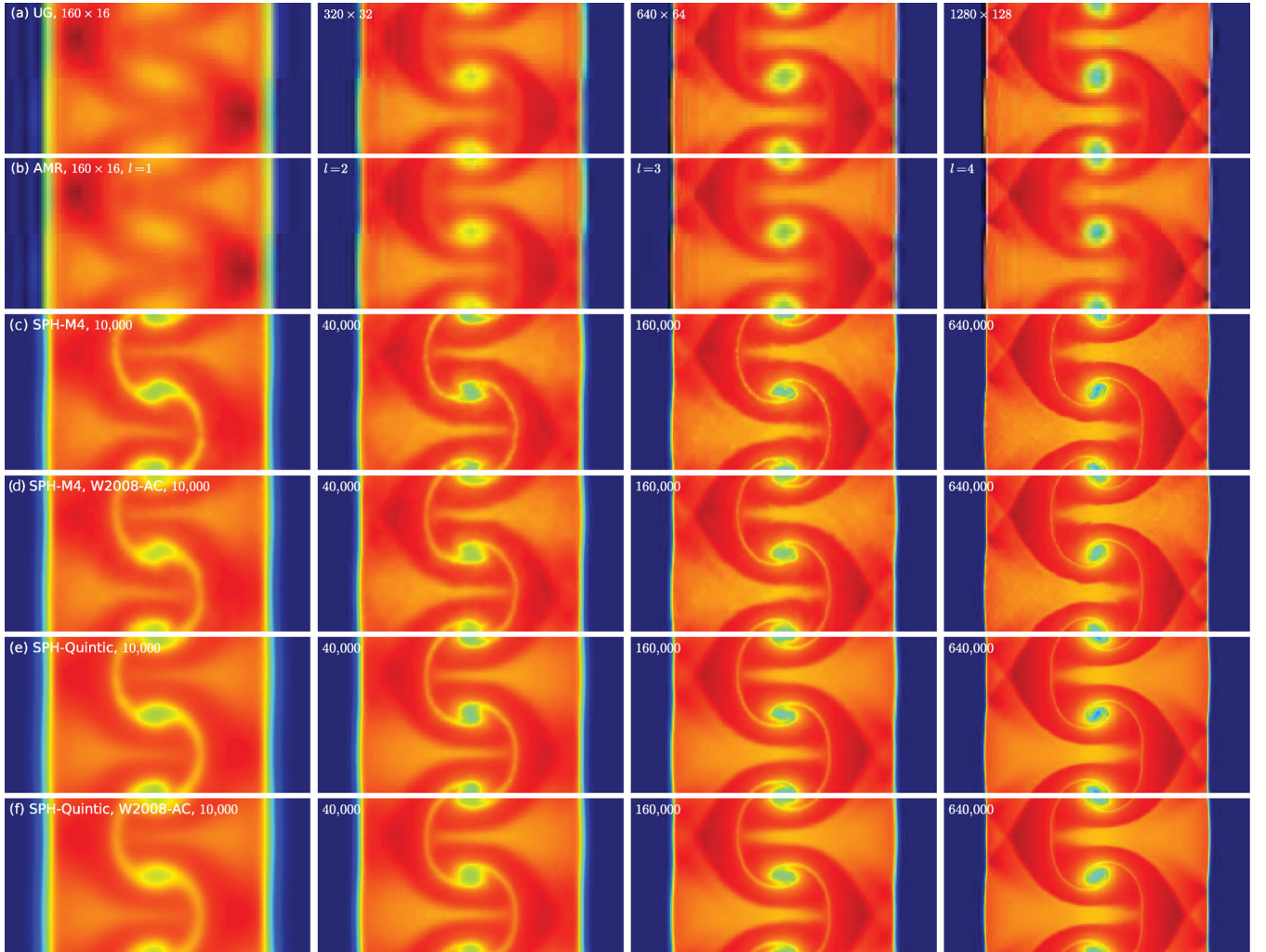
Figure 5. The density structure of the \mathcal{M}' = 2 non-linear thin shell instability in the range -1 < x < +1 , 0 < y < 1 at a time t = 1.2 modelled with (a) MG using uniform grid, (b) MG using AMR with 1, 2, 3 and 4 refinement levels, (c) SEREN using the M4 kernel, (d) SEREN using the M4 kernel and the Wadsley et al. (2008) conductivity, (e) SEREN using the quintic kernel, (f) SEREN using the quintic kernel and the Wadsley et al. (2008) conductivity. The left-hand column shows the NTSI using the smallest resolution ( 160 \times 16 cells for the finite volume code and N = 10\,000 for the SPH code) with increasing resolution moving right to the highest resolution ( 1280 \times 128 for the finite volume code and N = 640\,000 particles for the SPH code). The AMR simulations have the same equivalent resolution as the corresponding uniform grid simulation in the above row. Each subfigure shows the density field (blue: low density; red: high density).
