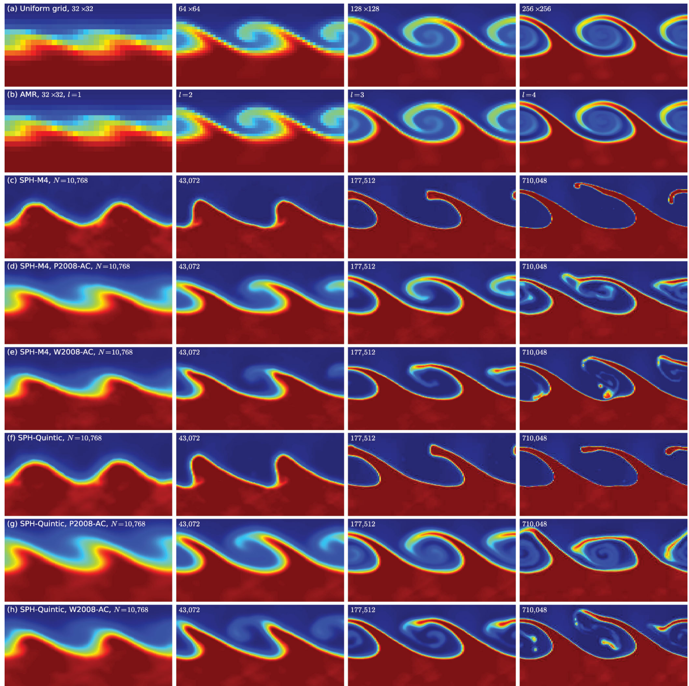
Figure 8. The density structure of the 10 : 1 KHI at a time t = \tau_{KH} = 1.74 modelled with (a) MG using uniform grid, (b) MG using AMR, (c) SEREN using the M4 kernel, (d) SEREN using the M4 kernel and the Price (2008) artificial conductivity, (e) SEREN using the M4 kernel and the Wadsley et al. (2008) conductivity, (f) SEREN using the quintic kernel, (d) SEREN using the quintic kernel and the Price (2008) artificial conductivity, (e) SEREN using the quintic kernel and the Wadsley et al. (2008) conductivity. The left-hand column shows the KHI using the smallest resolution ( 32 \times 32 cells for the finite volume code and N = 10\,768 for the SPH code) with increasing resolution moving right to the highest resolution ( 256 \times 256 for the finite volume code and N = 710\,048 particles for the SPH code). Note that we only show the top half of the computational domain ( y > 0 ) due to the symmetry of the initial conditions. Each subfigure shows the density field (blue: low density; red: high density).
