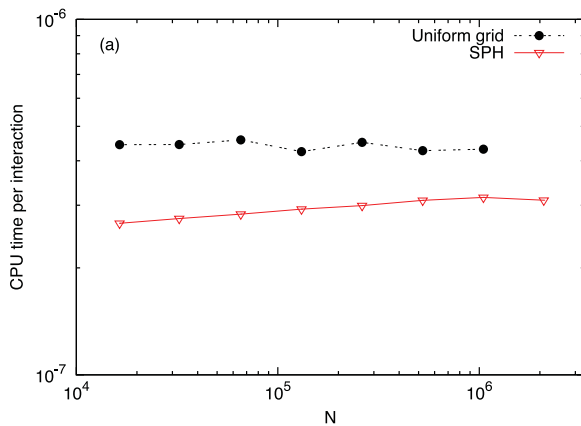
Figure 9. (a) The CPU time per cell–cell, or particle–particle, interaction in the finite volume and SPH codes. (b) The total CPU time of all cells or particles per time-step for the finite volume and SPH codes. The trend expected for constant no. of operations per cell/particle ( t_{\text{CPU}} \propto N ) is shown for reference.
