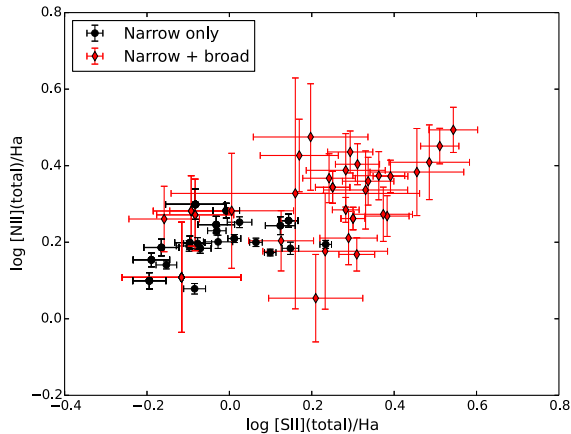
Figure 6. Comparison of the [S\ II]/H\alpha line ratio against the [N\ II]/H\alpha line ratio. To avoid errors associated with fitting multiple Gaussian components to blended emission lines, we have calculated the ratios using the total [S\ II] \lambda 6716 + \lambda 6731 and [N\ II] \lambda 6548 + \lambda 6583 fluxes. The line ratios for regions where only narrow components were fitted are shown in the black circles while the red diamonds show the line ratios calculated by adding both the narrow and broad components.
