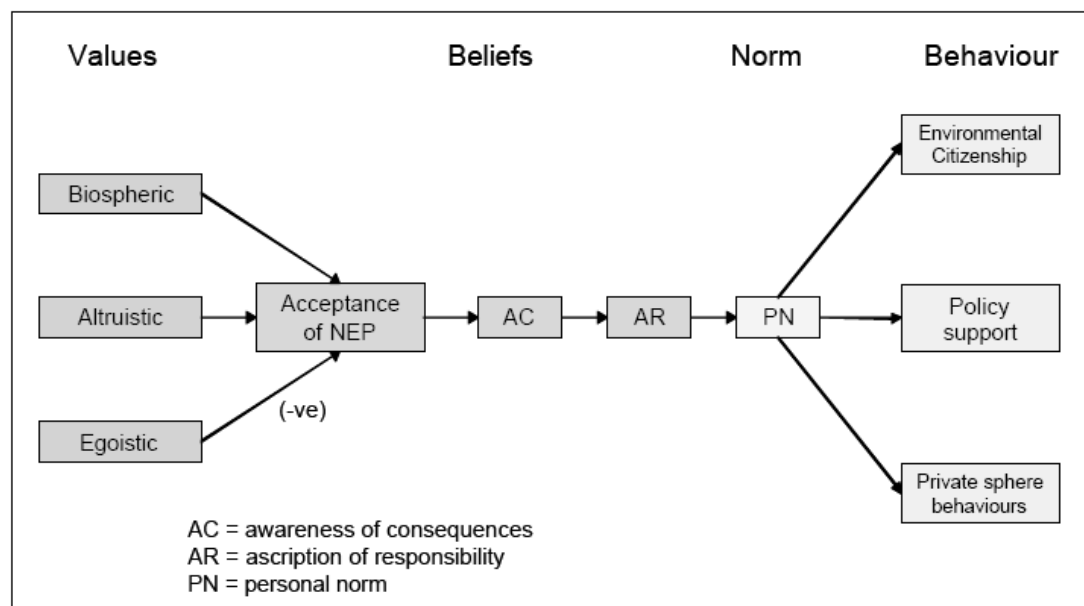
Figure 1: VBN Model
