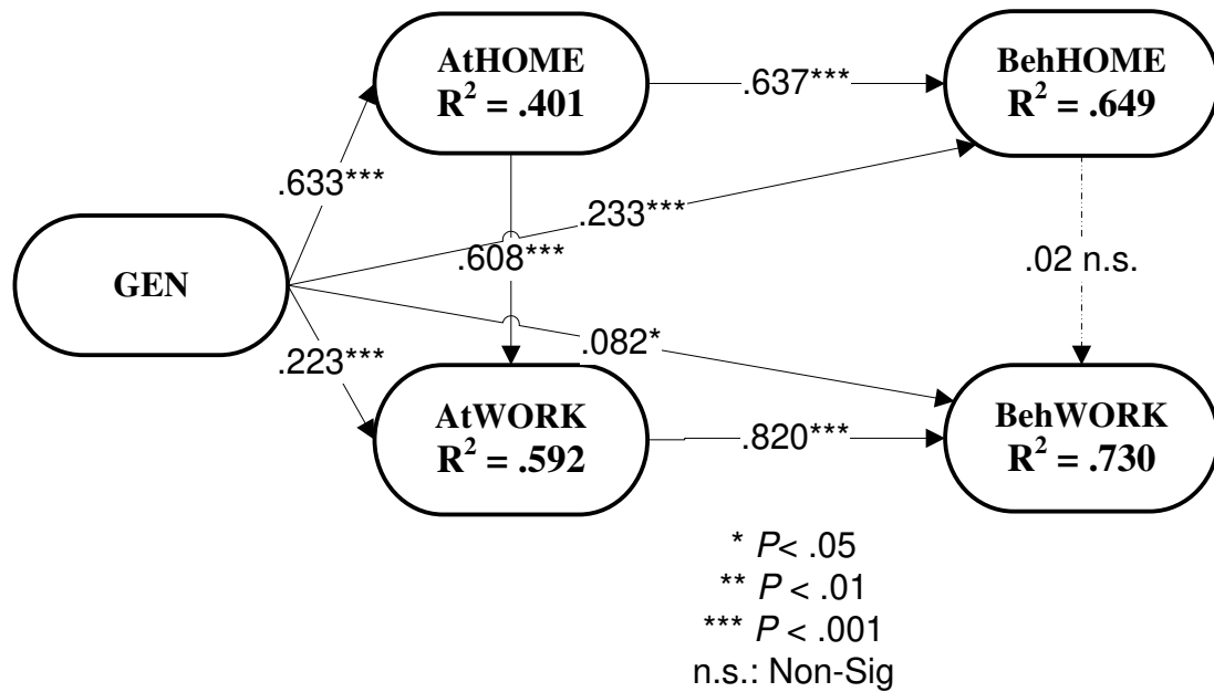
Figure 2: Research model with only direct effects demonstrated (standardised solution).
