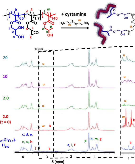
Figure 3. ^1\text{H} NMR spectra ( \text{CD}_3\text{OD} ) obtained for cystamine-derivatized \text{P}(\text{GMA}_{65}\text{-stat-GlyMA}_{1.7})\text{-HPMA}_{140} worm gels functionalized at 10 % w/w copolymer using a diamine/epoxy molar ratio of zero, 2.0 immediately after cystamine addition (e.g. prior to significant epoxy ring-opening), 2.0, 10 or 20. Each worm gel was reacted at 10 % w/w solids at 22 °C for 24 h. Expansion of the 2.6–3.4 ppm region is shown, indicating loss of epoxide signals and the appearance of four new broad (polymeric) cystamine signals at 3.0 – 3.2 ppm.
