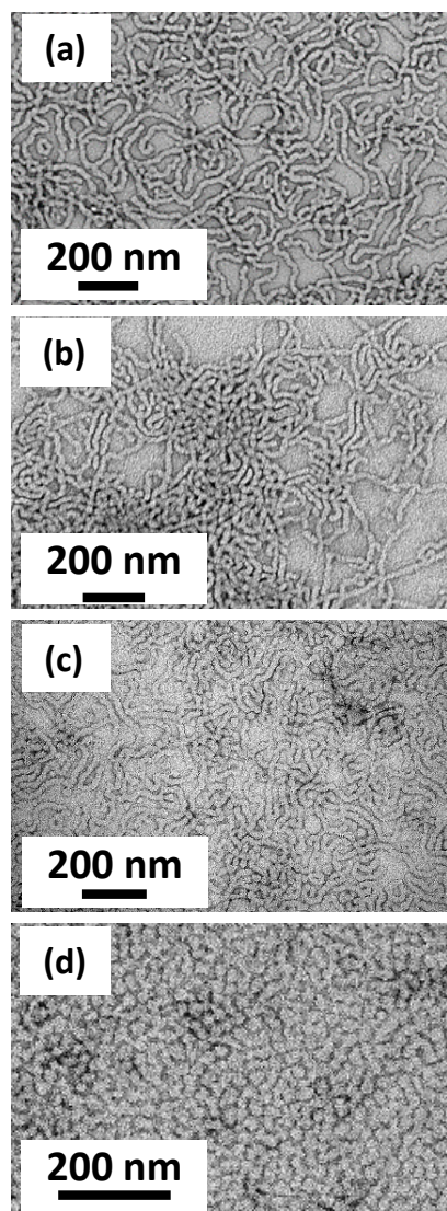
Figure 7. Representative TEM images recorded for: (a) PGMA 62 -PHPMA 140 worms (control); (b) P(GMA 65 - stat -GlyMA 1.7 )-PHPMA 140 worms prior to cystamine derivatization; (c) P(GMA 65 -GlyMA 1.7 )-PHPMA 140 worms dried from acidic aqueous solution (pH 2) after derivatization using a diamine/epoxy molar ratio of 0.05; (d) mixture of P(GMA 65 - stat -GlyMA 1.7 )-PHPMA 140 spheres and short worms obtained under the same conditions after derivatization using a diamine/epoxy molar ratio of 15.
