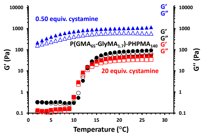
Figure 8. Oscillatory rheology studies showing storage moduli ( G' , filled symbols) and loss moduli ( G'' , open symbols) obtained on cooling 10 % w/w aqueous dispersions of precursor (black circles) and cystamine-functionalized P(GMA 65 - stat -GlyMA 1.7 )-PHPMA 140 worm gels, with the latter being prepared at pH 8-9 using diamine/epoxide molar ratios of either 0.50 (blue triangles) or 20 (red squares).
