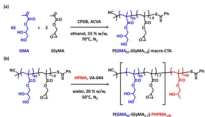
Scheme 1. (a) Synthesis of poly(glycerol monomethacrylate- stat -glycidyl methacrylate) [P(GMA 65 - stat -GlyMA 1.8 )] macro-CTA via statistical copolymerization of GMA and GlyMA using 2-cyano-2-propyl benzodithioate (CPDB) RAFT agent and 4,4'-azobis(4-cyanovaleic acid) (ACVA) initiator (CTA/ACVA molar ratio = 5.0) at 55 % w/w solids in ethanol at 70 °C. (b) Synthesis of poly(glycerol monomethacrylate- stat -glycidyl methacrylate)-poly(2-hydroxypropyl methacrylate) [P(GMA 65 - stat -GlyMA 1.7 )-PHPMA 140 ] diblock copolymer via RAFT aqueous dispersion polymerization of HPMA at 50 °C and pH 6–7 using a P(GMA 65 - stat -GlyMA 1.8 ) macro-CTA at 20 % w/w solids (CTA/VA-044 = 4.0). The modest reduction in GlyMA content from 1.8 mol % to 1.7 mol % is the result of in situ ring-opening of the epoxide group by water, which affords GMA residues.
