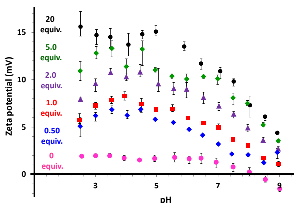
Figure 5. Zeta potential vs. pH measurements obtained for the unmodified copolymer precursor (0 equiv.) and cystamine-derivatized P(GMA 65 -stat-GlyMA 1.7 )-PHPMA 140 worms prepared using diamine/epoxy molar ratios of 0.50, 1.0, 2.0, 5.0 or 20. All pH titrations were performed from high pH to low pH. Error bars indicate one standard deviation. Positive zeta potentials observed at low pH are ascribed to protonation of the secondary amine groups formed during cystamine derivatization.
