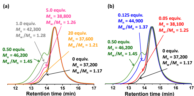
Figure 2. DMF GPC chromatograms obtained for the original (black traces) and cystamine-derivatized \text{P}(\text{GMA}_{65}\text{-stat-GlyMA}_{1.7})\text{-PHPMA}_{140} worm gels. Cystamine derivatization was conducted at 10 % w/w copolymer for 24 h at 22 °C using (a) excess cystamine (diamine/epoxide molar ratio = 1.0, 5.0 or 20) or (b) sub-stoichiometric cystamine (diamine/epoxide molar ratio = 0.50, 0.125 or 0.05), with equimolar cystamine (diamine/epoxide molar ratio = 0.50) included for comparison in each case (see green GPC traces). [N.B. In practice, the cystamine reagent may also react with the RAFT end-groups which means that the equimolar condition is only an approximation.]
