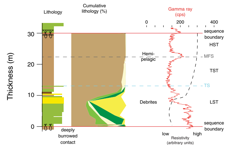
Figure 12. Idealized bottomset succession from the Miocene clinothems, based on sequence m5.45 at Site M29. Note the impact of the high glauconite content on the trace of the gamma ray logs (in cps, counts per second), which obscures the lithological pick of the sequence boundary (red line) (Inwood et al., 2013). See Figure 4 for color and symbol explanation. HST, TST, LST—highstand, transgressive, and lowstand systems tract, respectively; MFS—maximum flooding surface; TS—transgressive surface.
