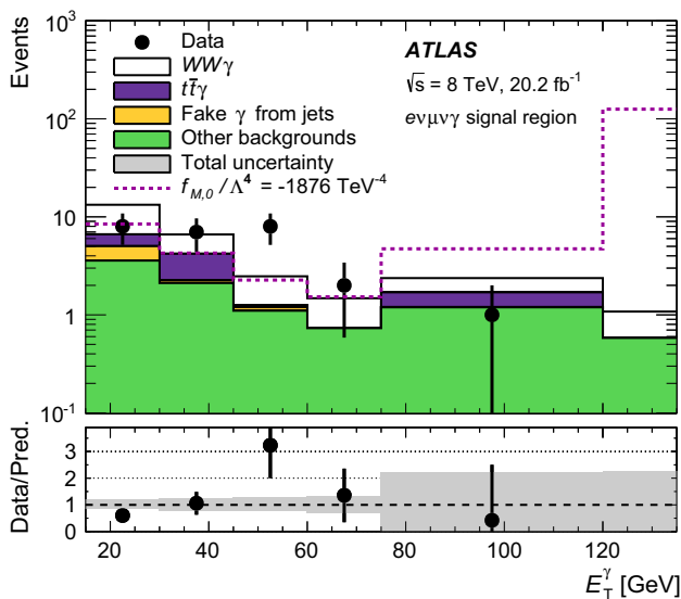
Fig. 3 Observed and expected transverse energy distribution of the photon with the highest E_T in the e\nu\mu\nu\gamma signal region. The data are shown together with the predicted signal and backgrounds. Also indicated is the expected event yield for a reference model describing aQGCs with f_{M,0}/\Lambda^4 = -1876 \text{ TeV}^{-4} (see Sect. 8). The last bin contains all overflow events. The lower panel shows the ratio of the observed number of events to the sum of expected signal and background events as well as the corresponding uncertainties
