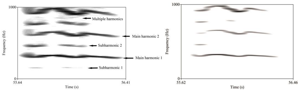
Figure 2: Narrow-band spectrogram of Kerry's sustained /a/ vowel at 35 dB (a: left) and 15 dB (b: right). The arrows on the image at 35 dB indicate the presence and position of the first two single subharmonics and main harmonics, and show the presence of multiple harmonics in the upper frequency range. At 15 dB, the subharmonics are visible at onset in the mid frequency range, and in the upper frequency range during in the medial portion of the vowel.
