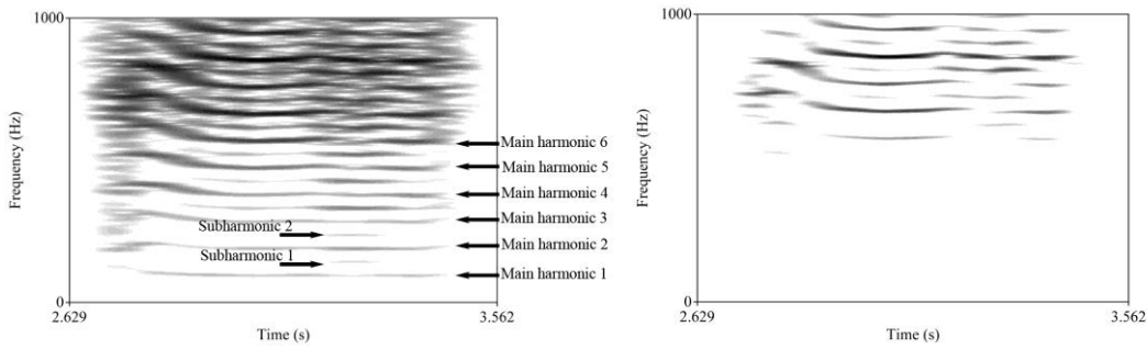
Figure 1: Narrow-band spectrogram of Andrew's sustained /a/ vowel at 35 dB (a: left) and 15 dB (b: right). The arrows on the image at 35 dB indicate the presence and position of the first two single subharmonics and the first six main harmonics. At 15 dB, the upper subharmonics and main harmonics remain visible in the 500-1000 Hz range only.
