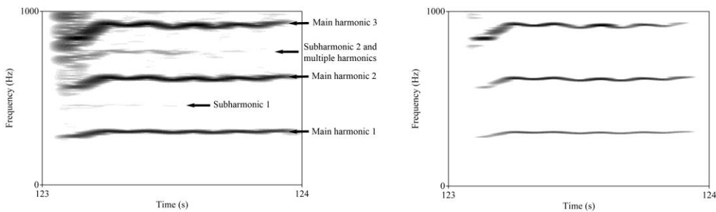
Figure 3: Narrow-band spectrogram of Rachel's sustained /a/ vowel at 35 dB (a: left) and 15 dB (b: right). The arrows on the image at 35 dB indicate the presence and position of the first two single subharmonics and three main harmonics. There are multiple harmonics in the upper frequency range, above subharmonic 2. At 15 dB, only the subharmonics above main harmonic 3 remain visible at onset.
