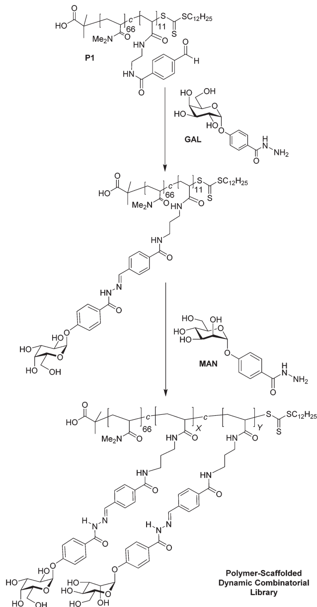
Scheme 1 Preparation of carbohydrate-functionalised PS-DCLs in 100 mM \text{NH}_4\text{OAc}-\text{AcOH} , pH 4.5, \text{D}_2\text{O} . PS-DCLs generated for templation with Con A were prepared in solutions which also contained 2 mM \text{CaCl}_2 , while PS-DCLs generated for templation with LTB were prepared in solutions containing 100 mM NaCl.
