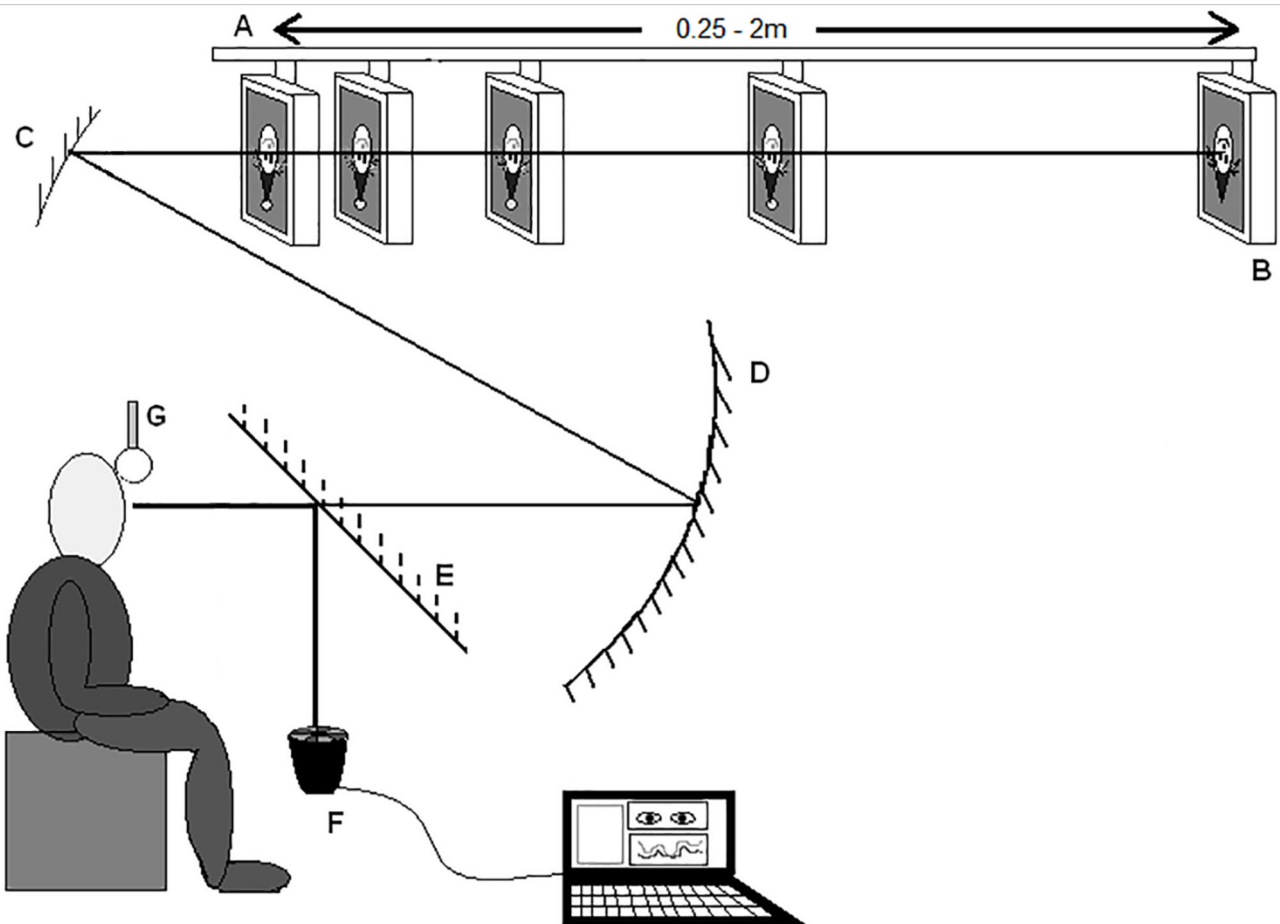
Figure 1 Infant vision laboratory. (A) Motorised beam. (B) Target monitor. (C) Upper concave mirror. (D) Lower concave mirror. (E) Hot mirror. (F) PlusoptiX S04 PowerRef II. (G) Headrest.
