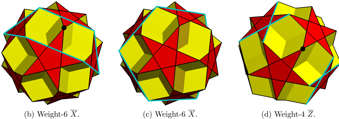
Figure 1: The smallest code based on a \{4, 5\} -tiling has parameters [[60, 8, 4]] and is related to the so called dodecadodecahedron . This can be seen as follows: We use the dual \{5, 4\} -tiling where four pentagons meet at every vertex. Half of the faces (red) are deformed into pentagrams with self-intersecting edges, see (a). Arranging the vertices on the surface of a sphere and allowing for self-intersecting faces, gives the dodecadodecahedron, see (b-d). A vertex is highlighted by a dot in order to show that one can label some of the logical operators by the 30 vertices (see Appendix B).
