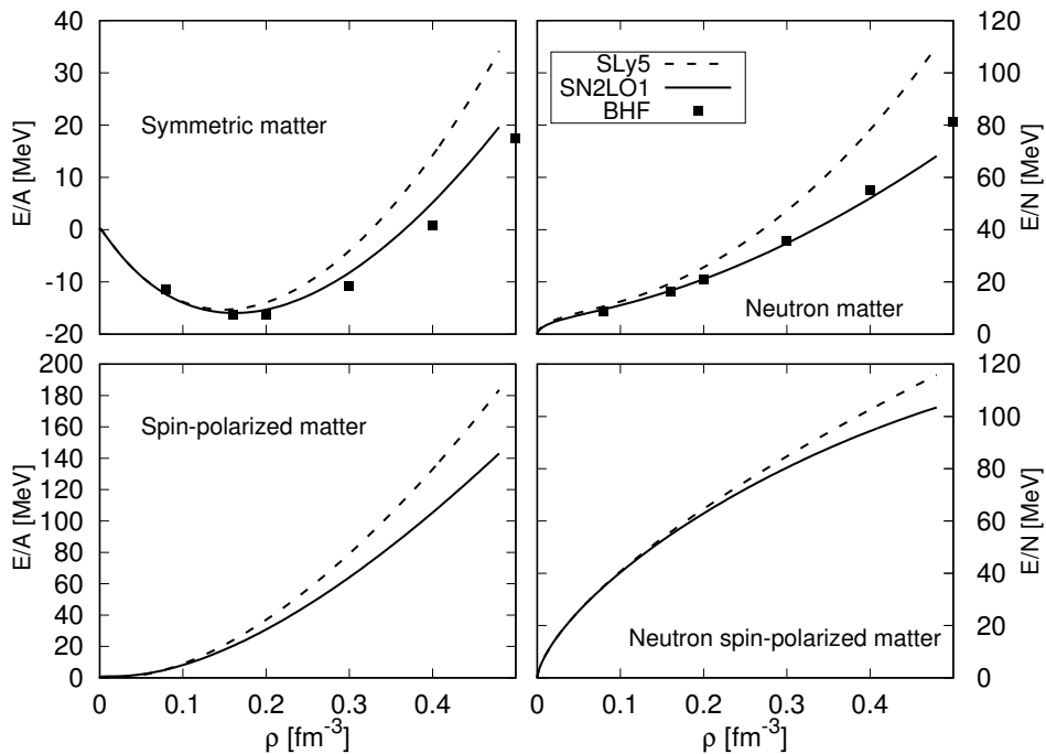
FIG. 9: (Colors online) Equation of state for SNM and PNM obtained with the N2LO Skyrme interaction. The squares represent the values obtained from BHF calculations.
