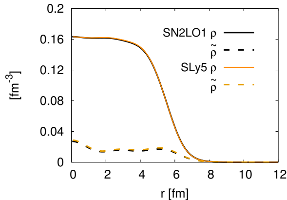
FIG. 6: (Colors online) Isoscalar particle density and pairing density for ^{120}\text{Sn} obtained with a self-consistent mean-field calculation with the SLy5 interaction.
