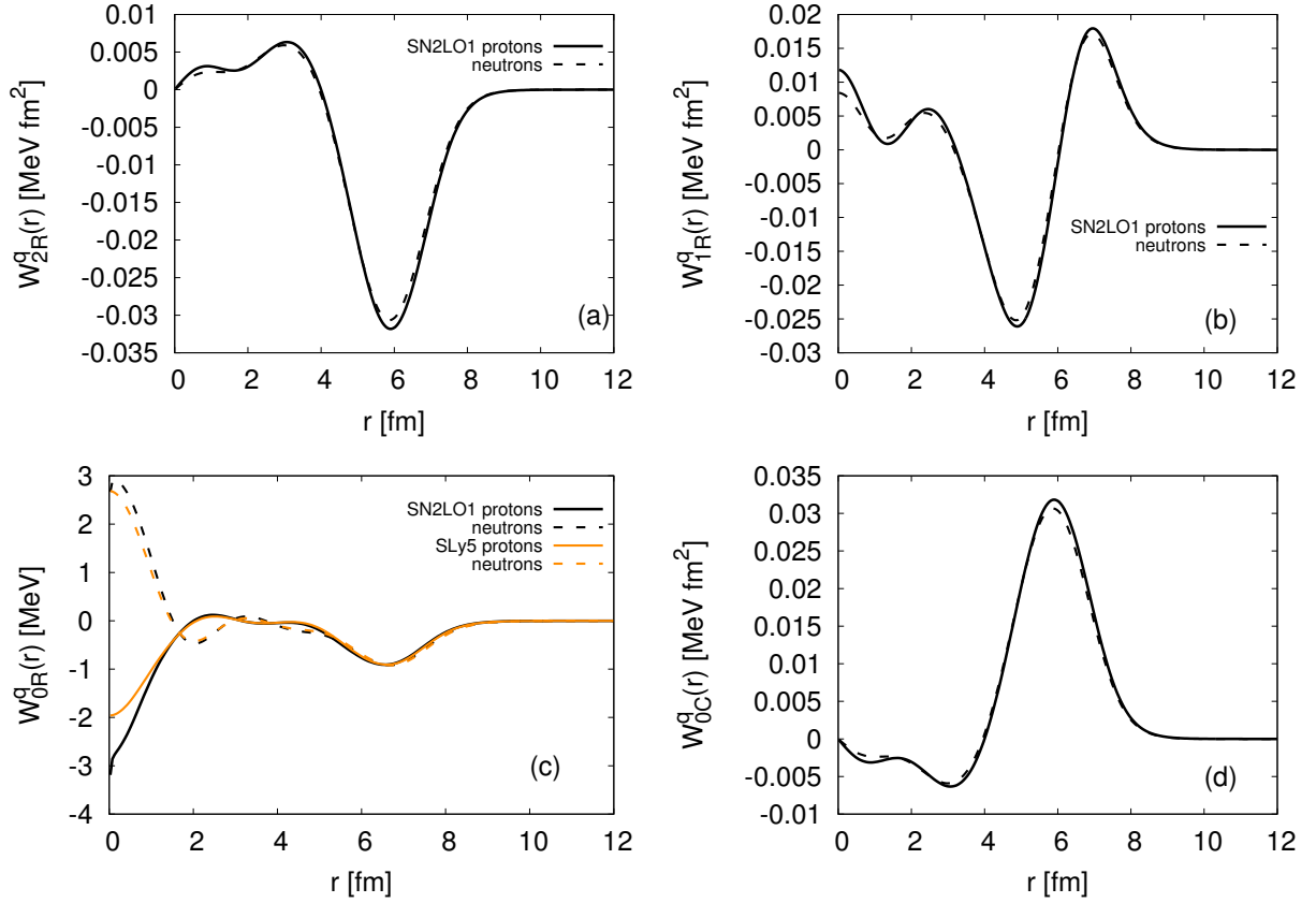
FIG. 4: (Colors online) Same as Fig. 2 but for the spin-orbit fields given in Eq. (32).
