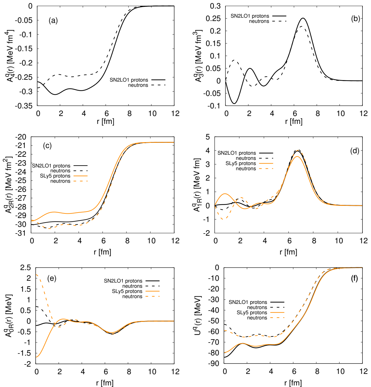
FIG. 2: (Colors online) Radial dependence of the coefficients defined in Eq. (32) for ^{208}\text{Pb} obtained using the SN2LO1 and SLy5 interactions. See text for details.
