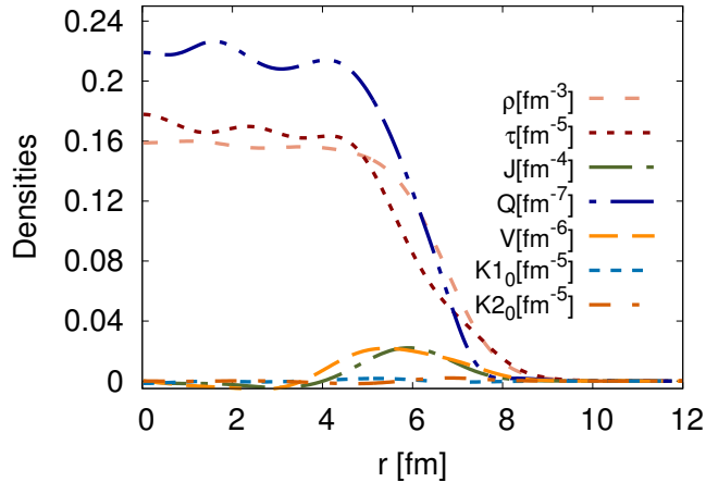
FIG. 1: (Colors online) Isoscalar densities in ^{208}\text{Pb} calculated using single particle wave functions obtained by a SLy5 mean-field solution. See text for details.
