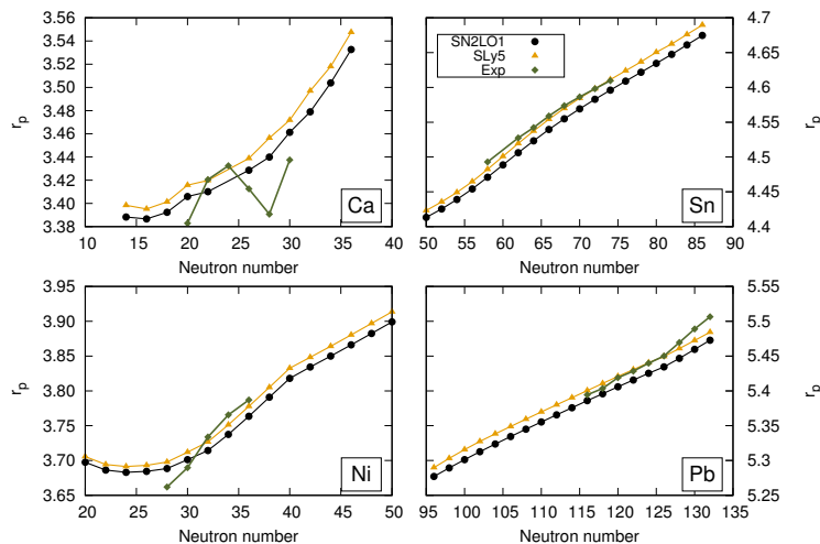
FIG. 14: (Colors online) Systematic comparison of proton radii. Experimental data are taken from Ref. [73].
