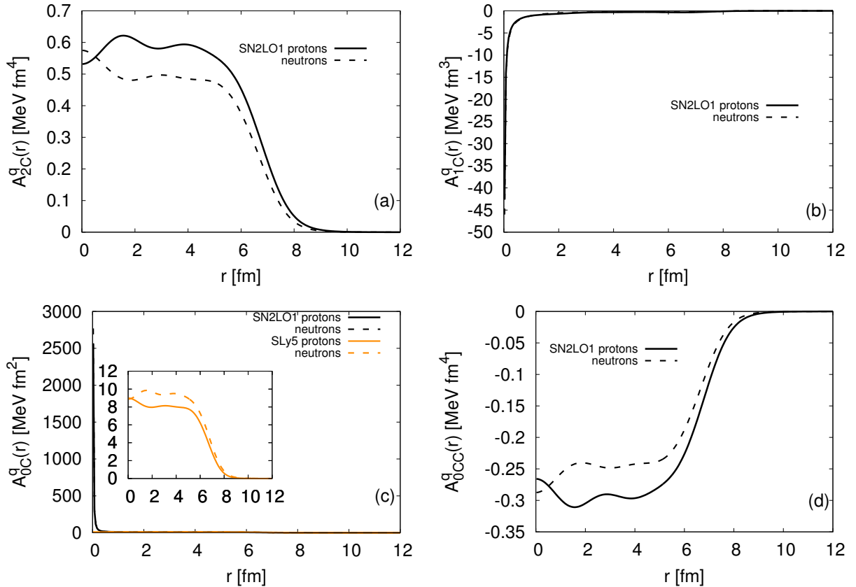
FIG. 3: (Colors online) Same as Fig. 2, but for centrifugal fields given in Eq. (32).
