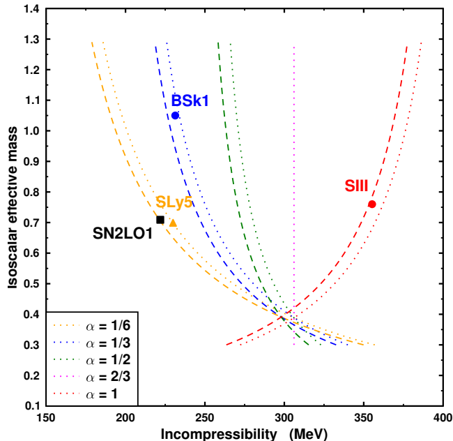
FIG. 10: (Colors online) Correlation between the effective mass and the nuclear incompressibility in infinite nuclear matter for different values of the power of the density dependent term. The curves correspond to different values of the power of the density dependence; dotted curves correspond to standard N1LO Skyrme EDF while dashed ones correspond to N2LO Skyrme EDF.
