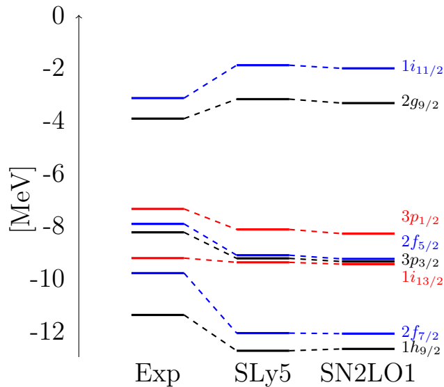
FIG. 16: Same as Fig. 15, but for ^{208}\text{Pb} .
