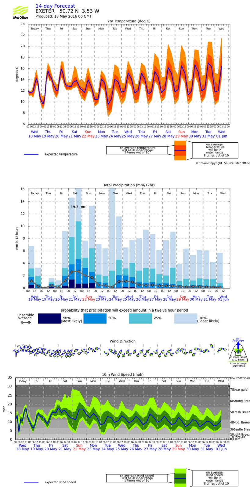
Fig. 6. Fourteen-day forecasts of temperature, precipitation and wind (top, middle and bottom panel, respectively) for Exeter, issued on 18 May 2016 at 06.00 GMT.
