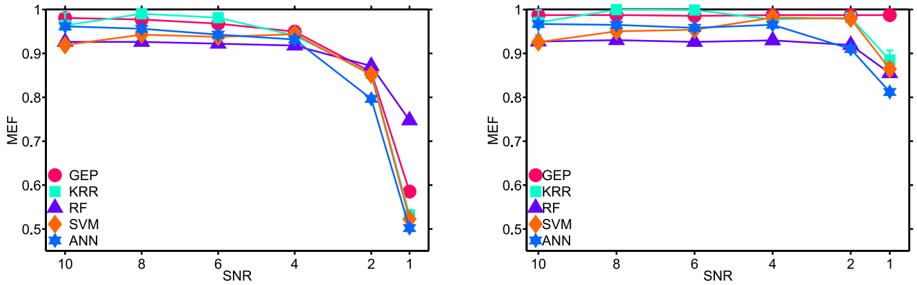
Figure 4. Effect of adding noise to original signal on prediction capacity for GEP, KRR, RF, SVM and ANN. The first panel contains the evolution of mean modelling efficiency (MEF) values from 20 independent runs for each increasing level of noise. MEF is computed after learning from a data set of 200 data points and validating against 1000 data points containing noise. The second panel shows the evolution of mean MEF values from 20 independent runs for each increasing level of noise where MEF is computed after learning from a data set of 200 data points and validating against noise-free 1000 data points generated from equation 15.
