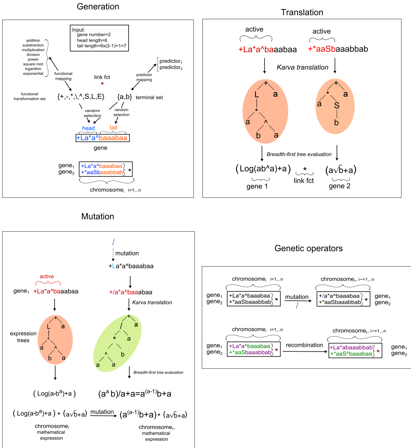
Figure 3. GEP evolution process components. A. Initial random generation of genes for creating chromosomes, the individuals evolved by GEP. B. GEP internal translation process from strings to expression trees and mathematical expressions. C. Changes made in the mathematical expression when applying the mutation operator on the genes of a GEP individual. D. Types of genetic operators for changing the GEP evolution individuals.
