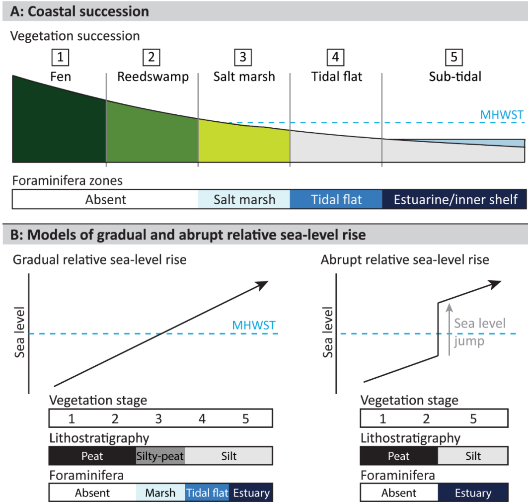
430 Figure 3: A: Model of northwest European coastal succession (after Waller et al., 1999). B: Models of 431 gradual (left) and abrupt (right) sea level rise as recorded by a coastal sequence (adapted after Long 432 and Shennan, 1994). Note: the length of panel B is not indicative of the amount of sedimentation and 433 both models assume the same total RSL rise.
