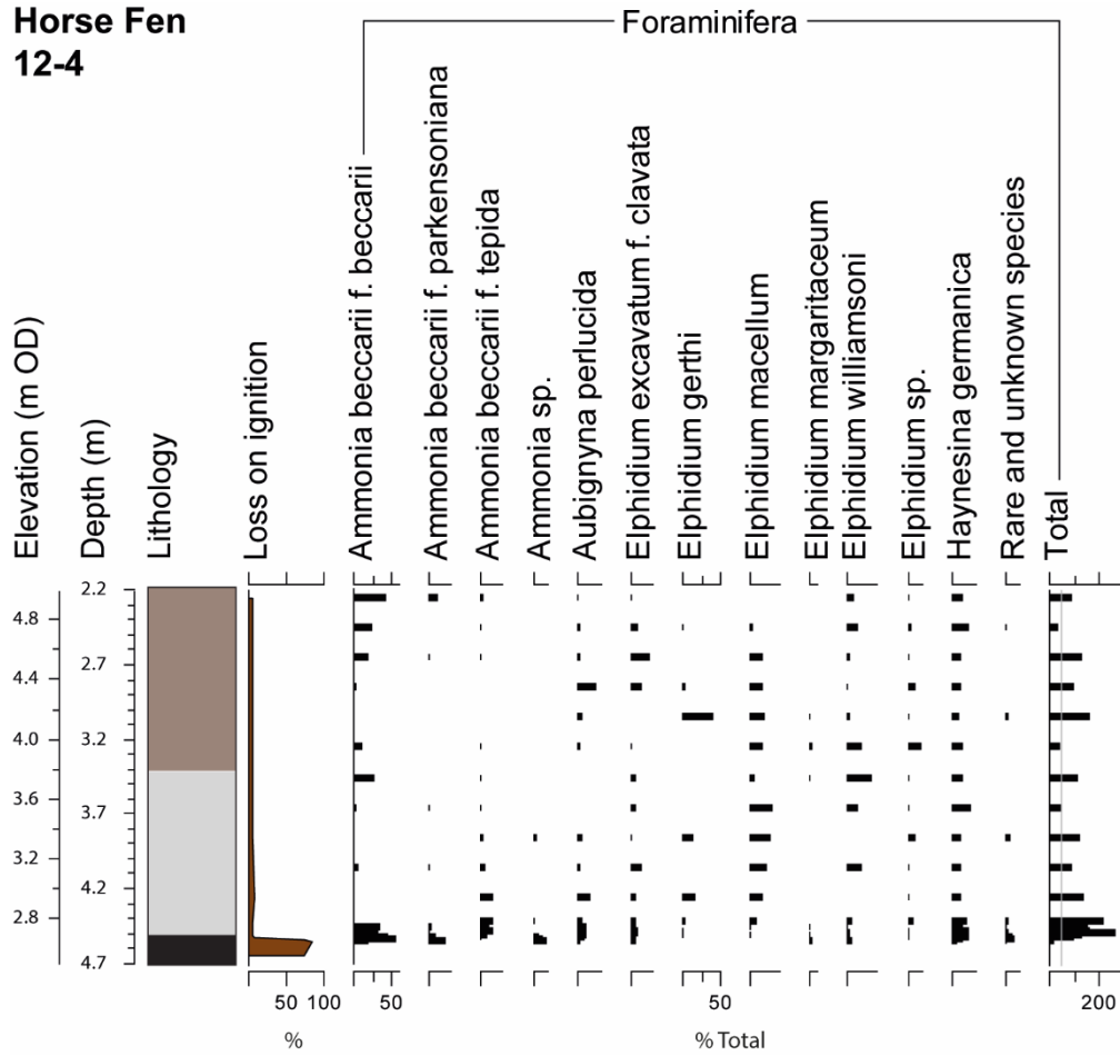
457 Figure 10: Horse Fen 12-4 litho- and bio-stratigraphy. Foraminifera >5% of total tests counted (grey line n=50). Lithology key same as Figure 6. Pollen for this 458 location in Stevens (1959) though exact elevations do not match.
