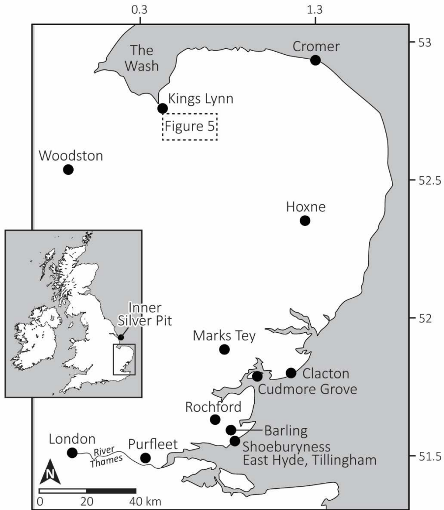
428 Figure 2: Map of eastern England showing location of the Nar Valley and key locations given in text.
