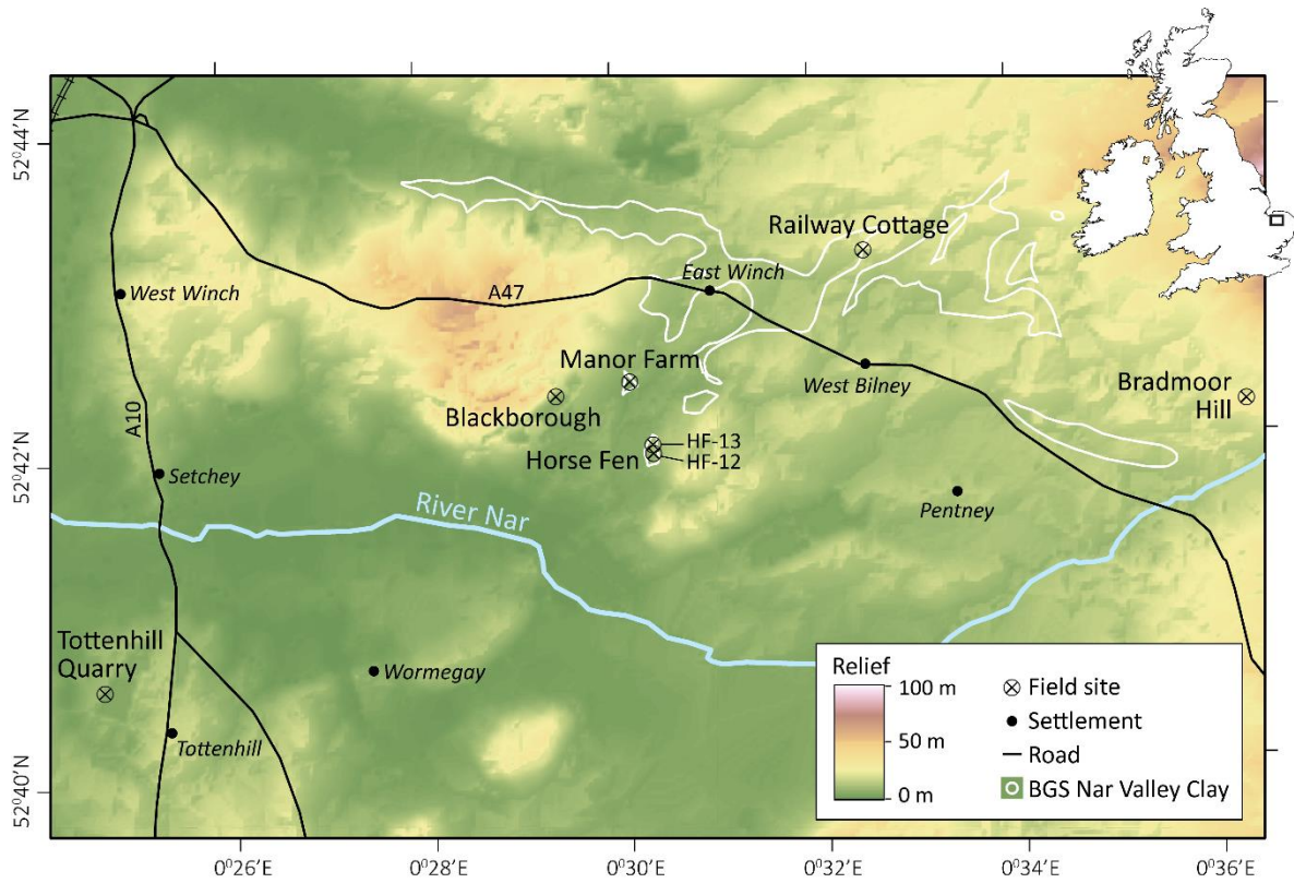
439 Figure 5: Map of the Nar Valley showing locations of new boreholes and key settlements. Topography 440 from NEXTMap British Digital Terrain Model Dataset Produced by Intermap with tickmarks in degrees, 441 minutes and second. White contours show location of Nar Valley Clay as mapped by British Geological 442 Survey (BGS).
