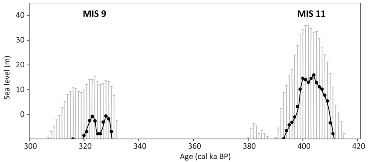
423 Figure 1: MIS 9 and 11 global sea level highstands recorded by the Spratt and Lisiecki (2016) ocean 424 core sea level stack (PC1) relative to present (0 m at 0 ka). Only vertical uncertainties shown, for 425 clarity.
