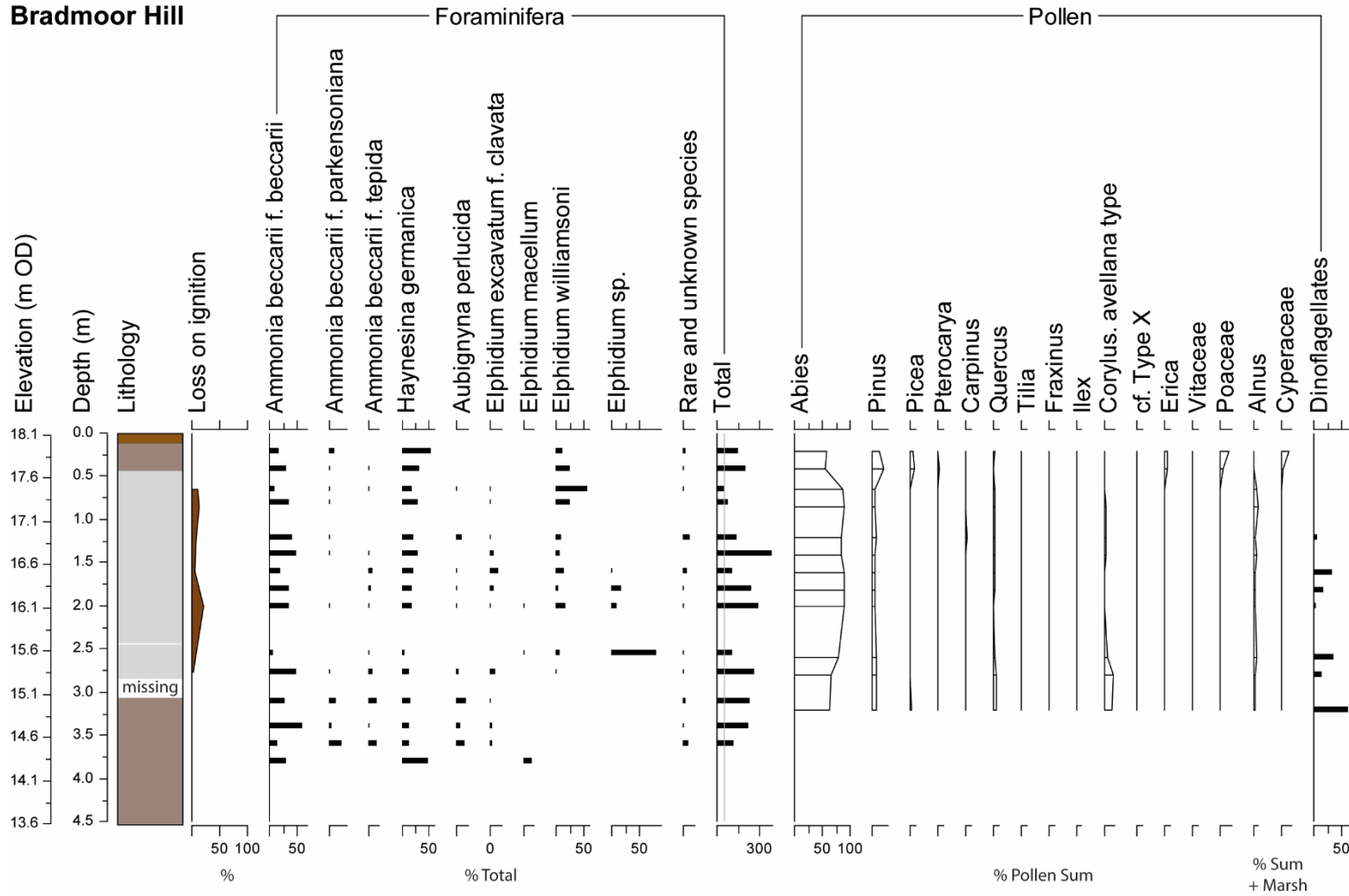
465 Figure 12: Bradmoor Hill litho- and bio-stratigraphy. Foraminifera >5% of total tests counted (grey line n=50). Selected pollen taxa shown. Lithology key same 466 as Figure 6.
