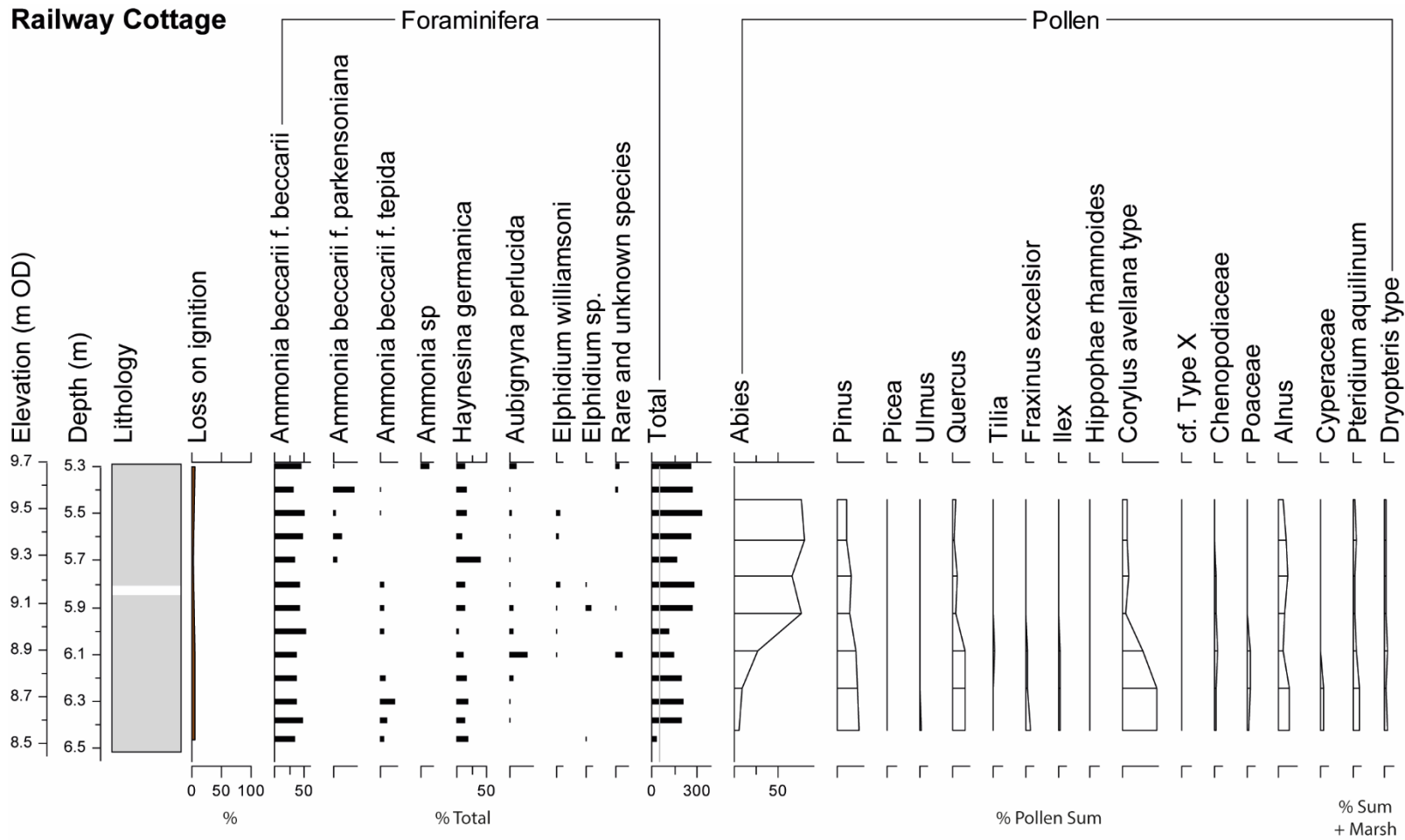
461 Figure 11: Railway Cottage litho- and bio-stratigraphy. Foraminifera >5% of total tests counted (grey line n=50). Selected pollen taxa shown. Lithology key 462 same as Figure 6.
