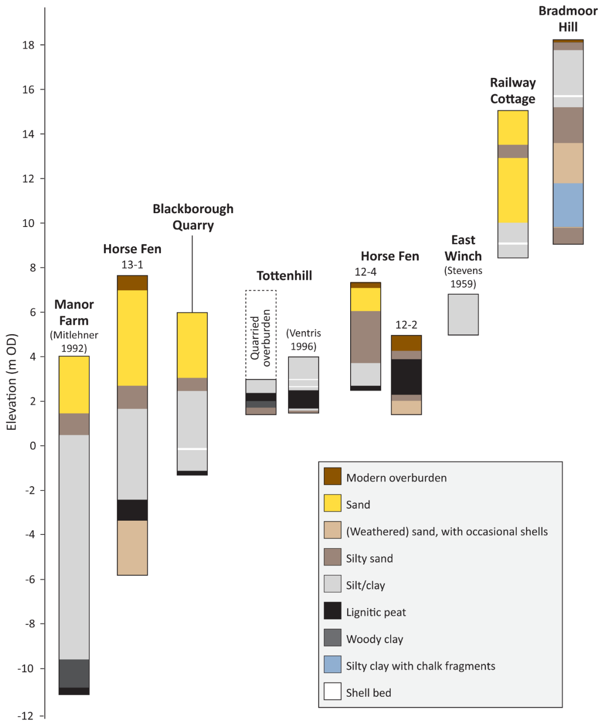
444 Figure 6: Nar Valley borehole lithology, collected as part of this work, with additional boreholes from 445 the literature at sites we were unable to resample. Elevation of Tottenhill section estimated from 446 Ventris (1996).
